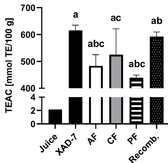
Figure 3. Total antioxidant capacity shown as Trolox equivalent (measured by Trolox equivalent antioxidant capacity (TEAC) assay) of pomegranate juice; XAD-7 extract; its anthocyanin (AF), copigment (CF), and polymeric fractions (PF); and the recombined extract (Recomb.). Results are presented as mean \pm SD of three independent experiments. For statistical analysis, one-way ANOVA followed by Tukey's multiple comparison test was performed. a: significantly different to juice with p < 0.05 ; b: significantly different to XAD-7 with p < 0.05 ; c: significantly different to Recomb. with p < 0.05 .
