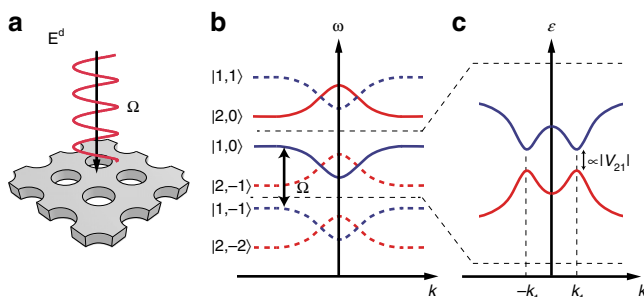
Fig. 1 Floquet bands and gaps in a periodically driven nonlinear photonic crystal. a Schematic of a nonlinear photonic crystal (PhC) placed in a monochromatic driving field \mathbf{E}^d at frequency \Omega . b Due to the periodic drive, static bands of the PhC (solid lines) create copies of themselves—Floquet bands (dashed lines)—by shifting up or down in the spectrum. c Two of the Floquet bands |1, m=0\rangle and |2, m=-1\rangle cross at \pm k_1 . Their coupling term V_{21} opens a new gap E_g —Floquet gap—and its size is linearly proportional to the magnitude of their coupling strength |V_{21}| under weak drive
