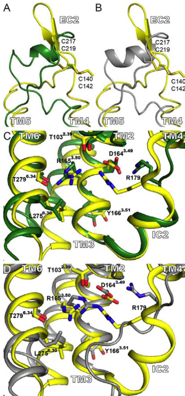
Figure 4. Structure of the EC2 and IC2. (A) and (B) Superposition of the EC2 for the crystal structure (yellow) and the 4T-hMOP-R (green) and 2T-hMOP-R (gray) models, respectively. The conserved disulfide bond between C140 in TM3 and C217 in EC2 is displayed. The numbers below correspond to the residue number for the equivalent residues in the human \mu opioid receptor (C219 and C142). (C) and (D) display views from the intracellular milieu, particularly interactions around the DRY motif. In (C) a comparison of the crystal structure (yellow) with 4T-hMOP-R (green) is shown. In (D) comparison of the crystal structure (yellow) with 2T-hMOP-R (gray) is shown. Relevant side chains are depicted.
