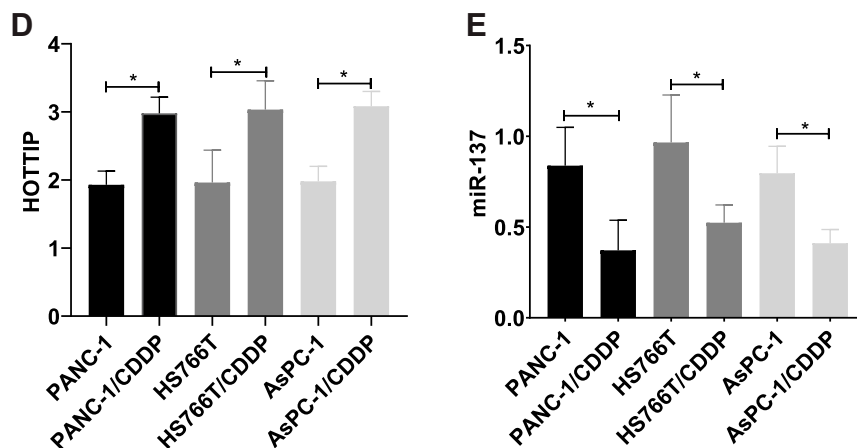
Figure 3 Construction results of cisplatin-resistant pancreatic cancer cell lines. (A) Growth inhibition of PANC-1/CDDP cells by different concentrations of cisplatin. (B) Growth inhibition of HS766T/CDDP cells by different concentrations of cisplatin. (C) Growth inhibition of AsPC-1/CDDP cells by different concentrations of cisplatin. (D) Expression changes of HOTTIP in pancreatic cancer drug-resistant cell lines. (E) Expression changes of miR-137 in pancreatic cancer drug-resistant cell lines. *Indicates that P < 0.05 .
