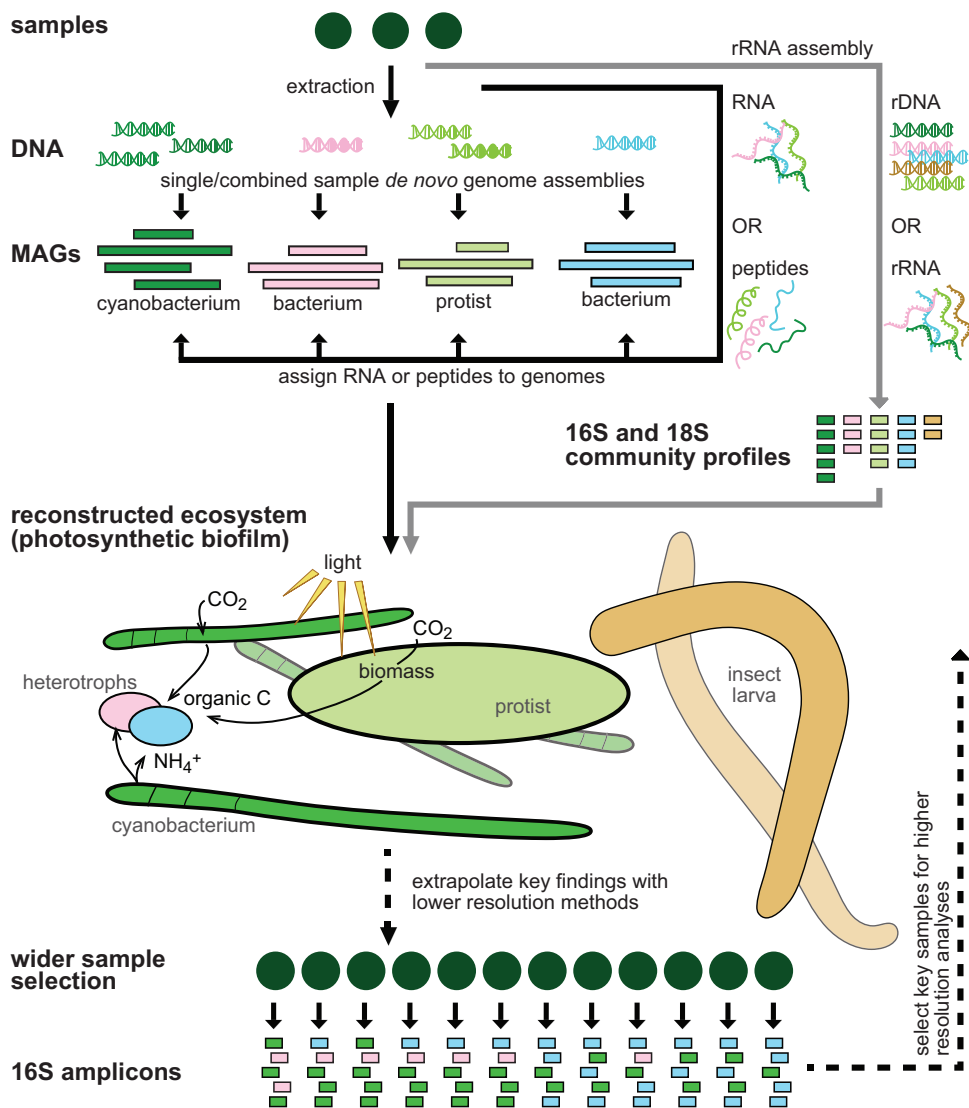
FIG 1 Schematic illustrating ecosystem reconstruction using functional genomics.
