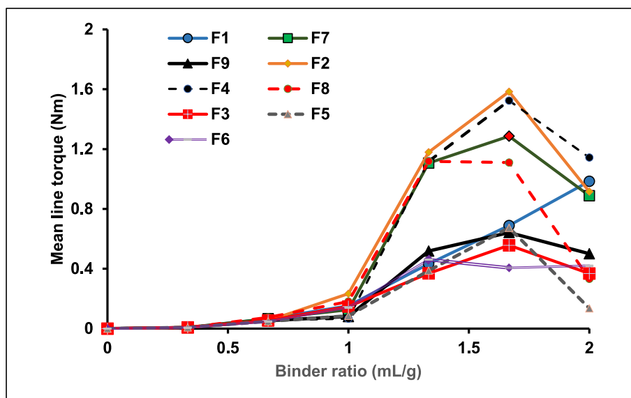
Fig. 4. Mean line torque of wet masses for tested Lisinopril SR pellets formulations.
