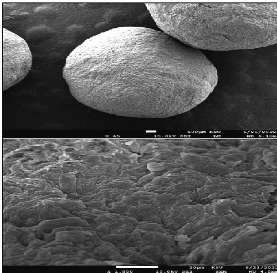
Fig. 9. Scanning electron micrographs of optimized LIS-SR matrix pellet formulation (A) and scanning electron micrographs of its surface (B).
