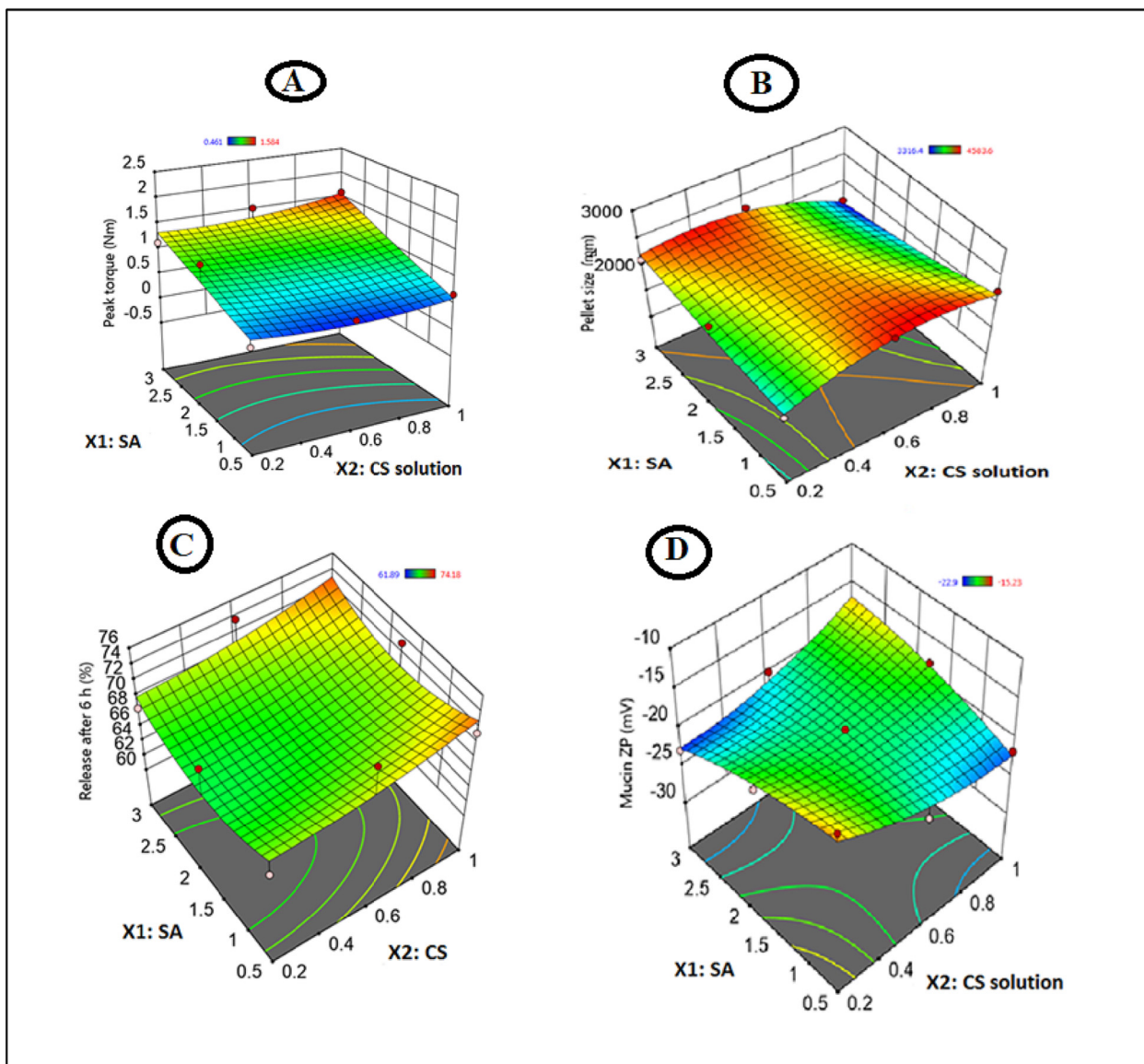
Fig. 6. Response surface plot estimating the effect of SA (X1) and CS solution (X2) on (A); the mean line torque value of pellet wet masses (Y1), (B); pellet sizes and (C); % Lisinopril release from SR pellets 6 h after and (D); mucoadhesion studies.
