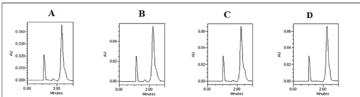
Fig. 3. HPLC chromatograms of LIS in HCl (chromatogram A), in phosphate buffer (chromatogram B), in Krebs solution (chromatogram C) and in water:methanol in ratio (7:3) (chromatogram D).
