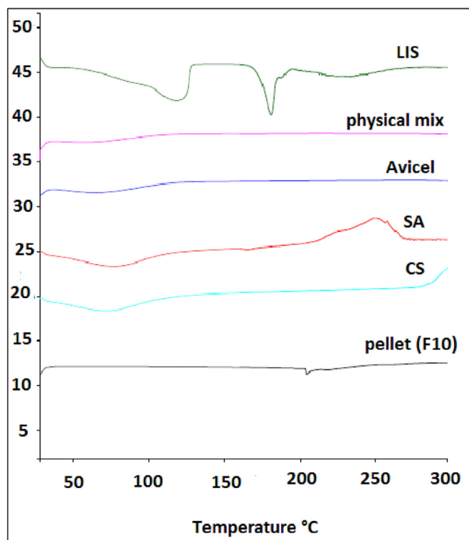
Fig. 10. DSC curve of untreated LIS, SA, CS, Avicel® and optimized LIS-SR matrix pellet formulation.
