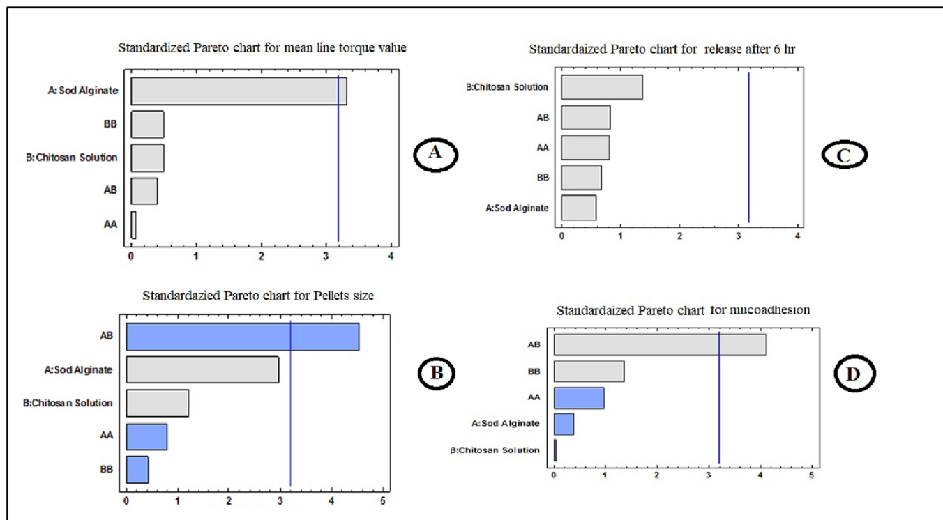
Fig. 5. Standardized Pareto chart estimating the effect of independent formulation factors on (A); mean line torque value of pellet wet masses, (B); pellet sizes and (C); % Lisinopril release from SR pellets 6 h after and (D); mucoadhesion studies.
