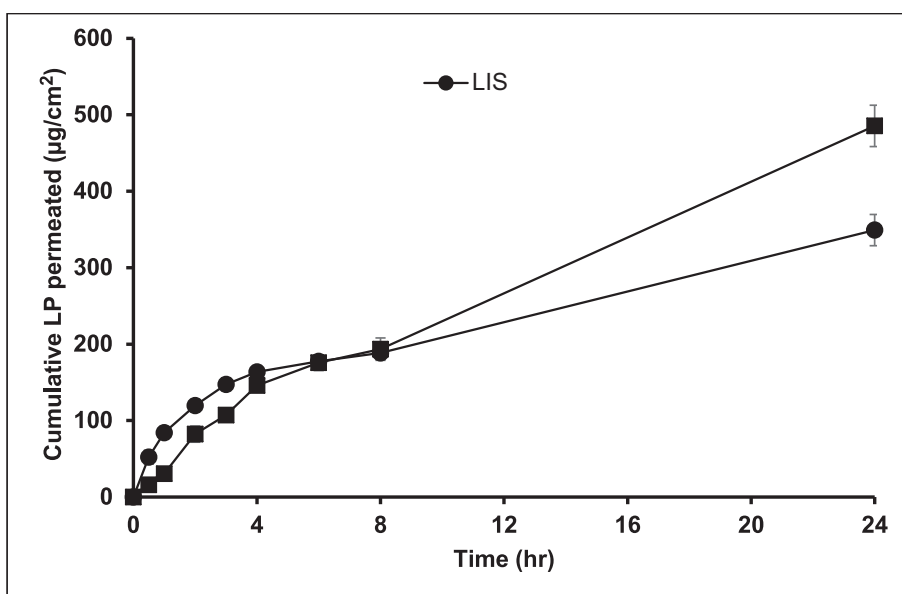
Fig. 12. Permeation profiles of LIS from the optimized LIS-SR matrix pellet formula compared to untreated drug (n = 6).
