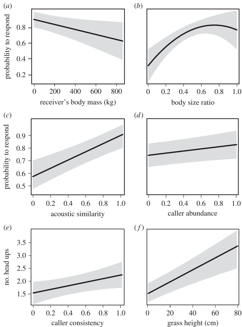
Figure 2. Probability of responding to an alarm call in relation to the body size of the receiver, the body size ratio between the caller and the receiver (H2), the acoustic similarity between caller and receiver alarms (H5) and the abundance of the caller (H4) ( a–d ). Head-up response to alarm calls in relation to the consistency of the caller (H3.1) and grass height (H6) ( e,f ). Body size ratio, acoustic similarity, abundance and consistency of the caller were all scaled between 0 and 1.
