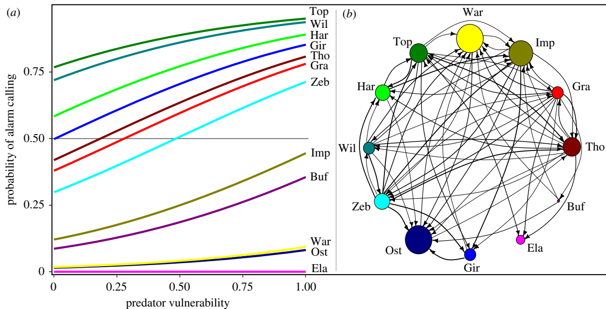
Figure 1. Communication network of African savannah herbivores. (a) Species-specific differences in the probability of alarm calling in relation to predator vulnerability. (b) Species-specific dependency on heterospecific alarm calls. Arrows point to species in which alarm calls elicited a response with edge weight representing response probability (cut-off point: 0.72). Node-size indicates the number of species whose alarm calls caused a response (for species abbreviations, see 'Study system'). (Online version in colour.)
