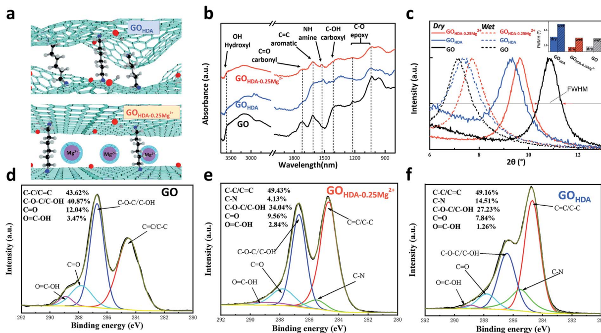
Fig. 1 (a) A schematic of \text{GO}_{\text{HDA-0.25Mg}^{2+}} and \text{GO}_{\text{HDA}} ; (b) FTIR spectra of GO, \text{GO}_{\text{HDA-0.25Mg}^{2+}} and \text{GO}_{\text{HDA}} ; (c) XRD spectra of GO, \text{GO}_{\text{HDA-0.25Mg}^{2+}} and \text{GO}_{\text{HDA}} ; X-ray photoelectron spectrometer spectra of (d) GO, (e) \text{GO}_{\text{HDA-0.25Mg}^{2+}} and (f) \text{GO}_{\text{HDA}} .
