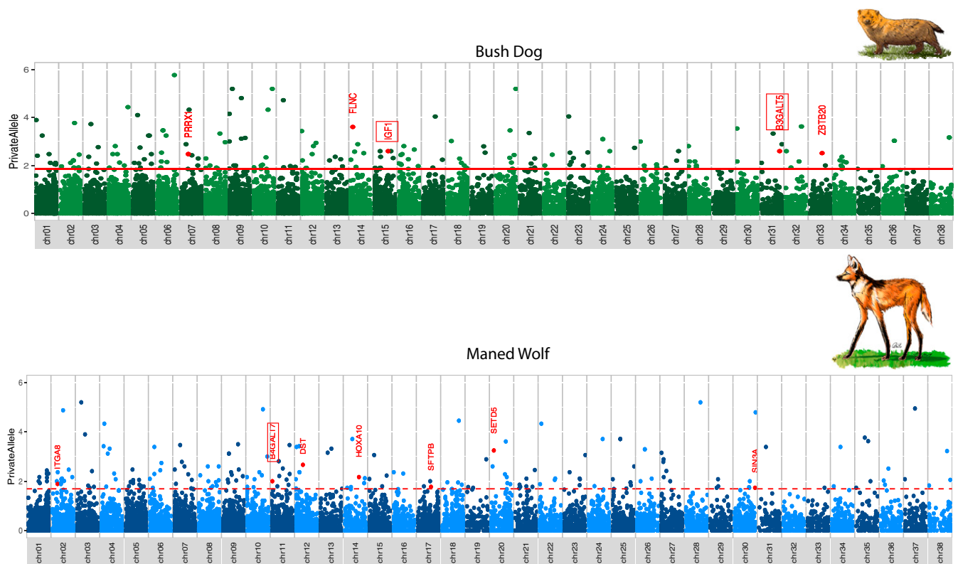
Fig. 6. Proportion of private alleles for the bush dog ( Top ) and maned wolf ( Bottom ) from 1-kb windows flanking 39,704 transcripts belonging to 32,704 genes. Significant genes ( P value <0.01) are shown above the horizontal red line. Genes involved in limb development are shown in red. Genes relevant to limb elongation are highlighted by a red rectangle.
