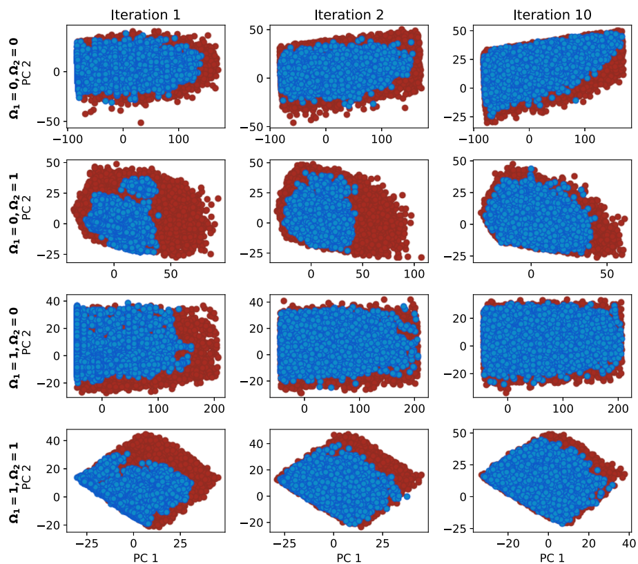
Fig. 15 The exploration of viable regions for the edge-triggered D flip-flop. \Omega_1 defines competitive (0) or noncompetitive (1) binding sites at promoter level, and \Omega_2 Michaelian (0) or linear (1) protein degradation form. Blue dots represent the viable solutions, red dots represent candidates for viable solutions
