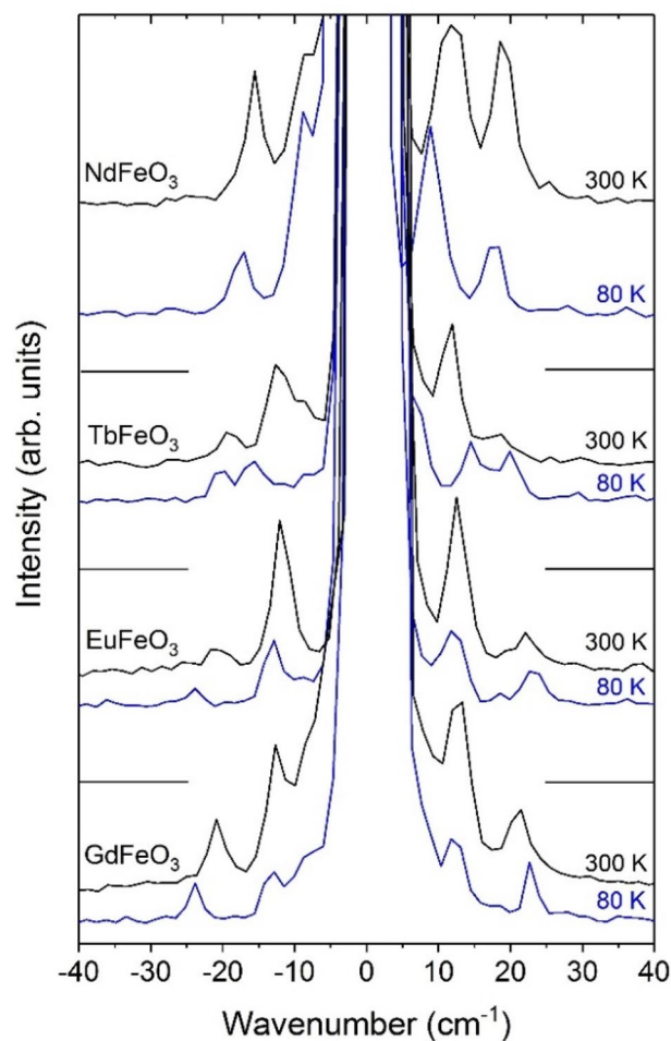
Figure 3. Representative unpolarized Stokes and anti-Stokes Raman spectra of R\text{FeO}_3 ( R = \text{Nd, Eu, Gd} and \text{Tb} ), in the -40 to 40 \text{ cm}^{-1} spectral range, recorded at 80 and 300 K.
