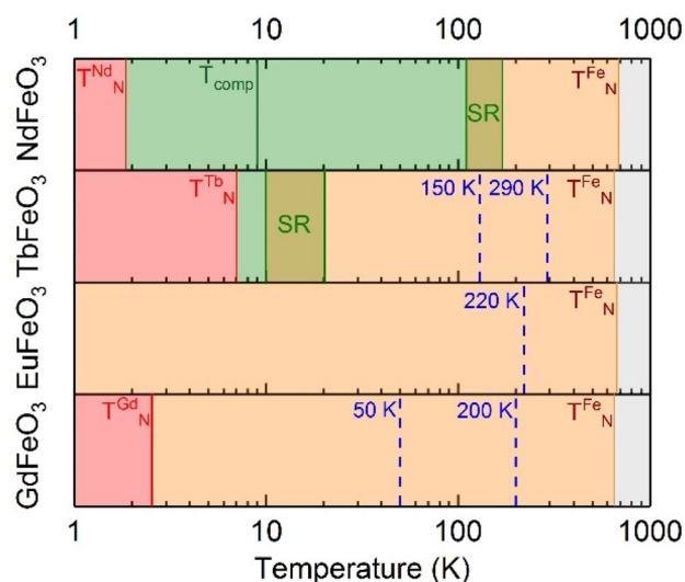
Figure 2. Magnetic phase sequence for R\text{FeO}_3 with R = \text{Nd}, \text{Tb}, \text{Eu} and \text{Gd} . Critical temperatures of the reported phase transitions taken from Refs. 10,13,25 . Dashed lines mark relevant anomalies observed in this work on M(T) curves, not associated with phase transitions.
