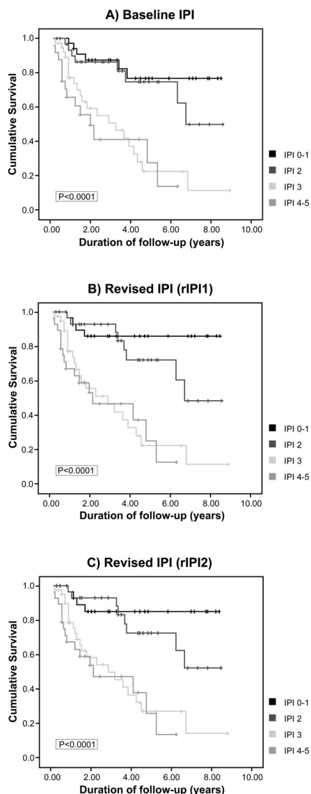
Figure 1 The three Kaplan Meier curves show differences in cumulative survival between with low-risk, low-intermediate, high-intermediate and high-risk categories using a baseline IPI model (A) and two revised IPI models. The first (rIPI1) incorporates flow cytometry and immunohistochemistry as routine staging (B) and the second IPI model (rIPI2) additionally incorporates molecular testing using IgH/IgL analysis (C).
