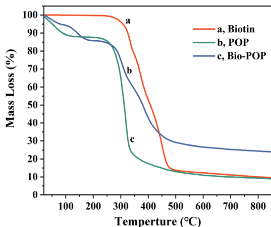
Fig. 5 TGA thermograms of biotin (a), POP (b) and Bio-POP conjugates (c) measured at 25 °C.
