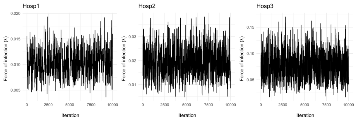
Figure S1 Markov Chain Monte-Carlo diagnostics
