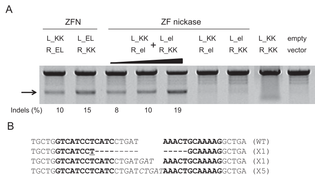
Figure 4. Two pairs of ZF nickases produce a DSB in the genome. (A) Nuclease or nickase-driven indels detected by T7E1 assay. PCR products amplified using genomic DNA from cells transfected with plasmids (4 μg/monomer) encoding nickases or nucleases were subjected to T7E1 digestion and analyzed by agarose gel electrophoresis. (Arrow) The expected position of the resulting DNA band. (The black triangle above the gel picture) The increase of the transfected plasmid (4, 8, and 10 μg/each monomer). (B) DNA sequences of the CCR5 wild-type and mutant clones. The two half-sites are shown in boldface letters. Microhomologies are underlined, and inserted bases are shown in italics. Dashes indicate deleted bases. The number of occurrences is shown in parentheses; X1 and X5 are the number of each clone. (WT) Wild type.
