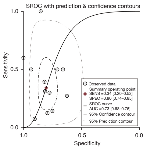
Figure 7 SROC curve of the diagnosis of T2 stage using EUS. SROC, summary receiver operating characteristic; AUC, area under curve; SENS, sensitivity; SPEC, specificity; EUS, endoscopic ultrasound.
