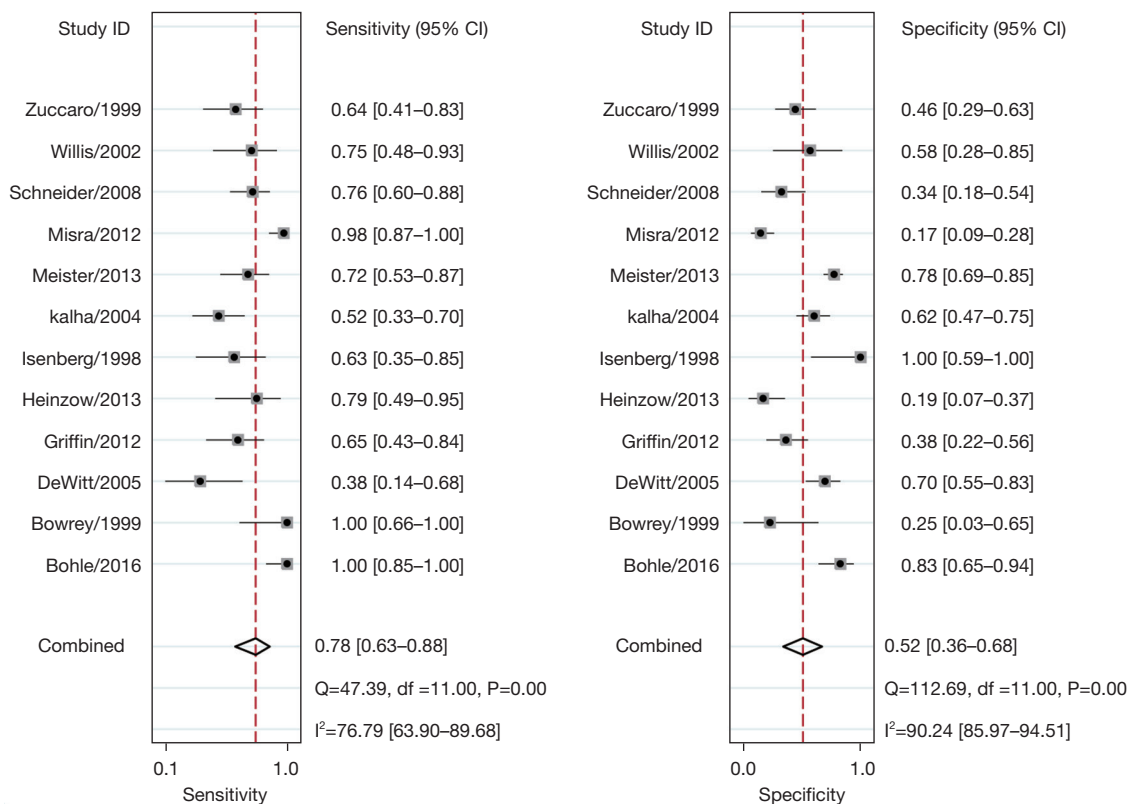
Figure 8 Forest plot of sensitivity and specificity of individual study and summary study on the diagnosis of T3 stage using EUS. CI, confidence interval; df, degree of freedom; EUS, endoscopic ultrasound.
