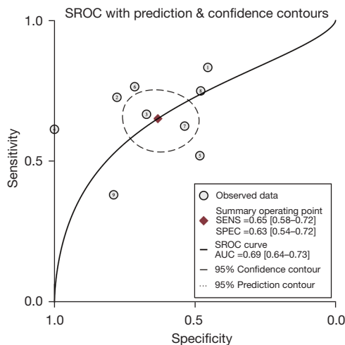
Figure 15 SROC curve of the diagnosis of N1 stage using EUS. SROC, summary receiver operating characteristic; AUC, area under curve; SENS, sensitivity; SPEC, specificity; EUS, endoscopic ultrasound.
