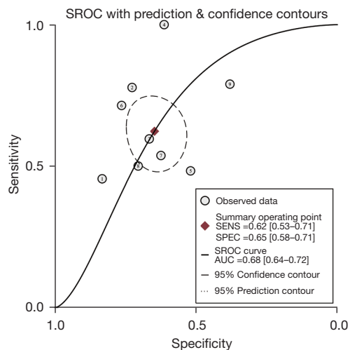
Figure 13 SROC curve of the diagnosis of N0 stage using EUS. SROC, summary receiver operating characteristic; AUC, area under curve; SENS, sensitivity; SPEC, specificity; EUS, endoscopic ultrasound.
