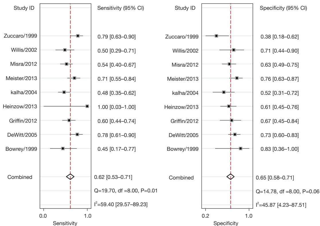
Figure 12 Forest plot of sensitivity and specificity of individual study and summary study on the diagnosis of N0 stage using EUS. CI, confidence interval; df, degree of freedom; EUS, endoscopic ultrasound.
