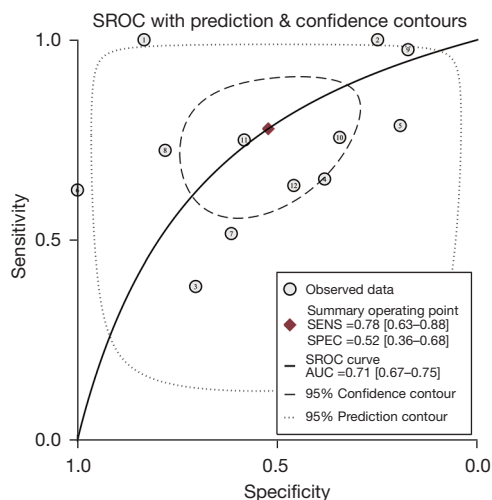
Figure 9 SROC curve of the diagnosis of T3 stage using EUS. SROC, summary receiver operating characteristic; AUC, area under curve; SENS, sensitivity; SPEC, specificity; EUS, endoscopic ultrasound.
