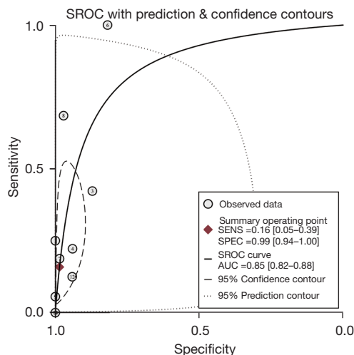
Figure 5 SROC curve of the diagnosis of T1 stage using EUS. SROC, summary receiver operating characteristic; AUC, area under curve; SENS, sensitivity; SPEC, specificity; EUS, endoscopic ultrasound.
