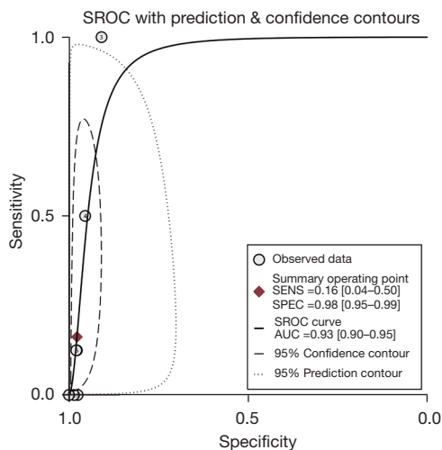
Figure 11 SROC curve of the diagnosis of T4 stage using EUS. SROC, summary receiver operating characteristic; AUC, area under curve; SENS, sensitivity; SPEC, specificity; EUS, endoscopic ultrasound.
