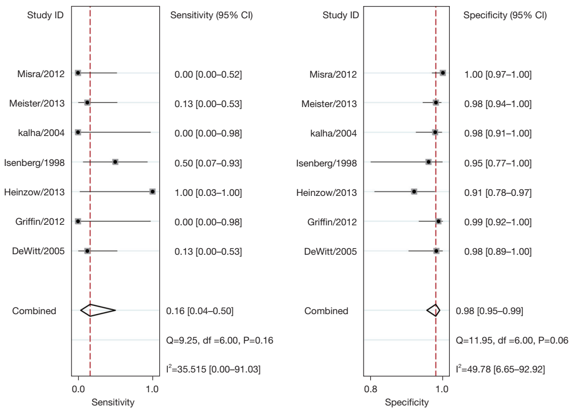
Figure 10 Forest plot of sensitivity and specificity of individual study and summary study on the diagnosis of T4 stage using EUS. CI, confidence interval; df, degree of freedom; EUS, endoscopic ultrasound.
