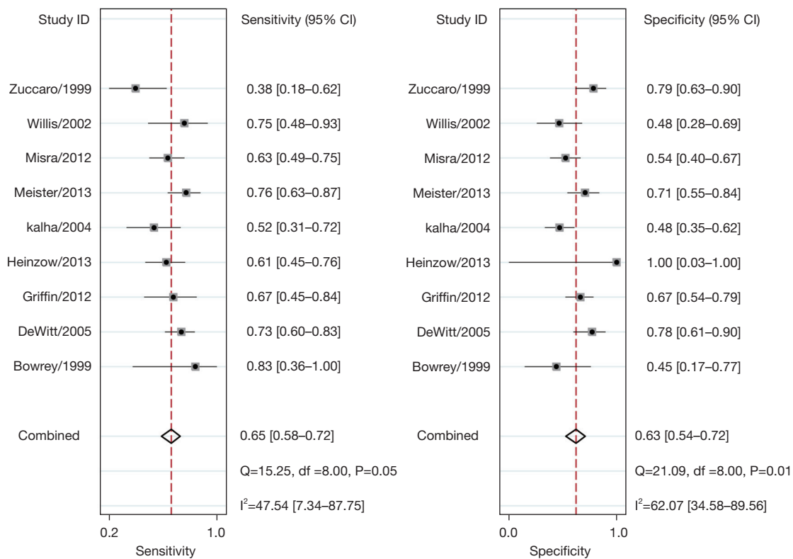
Figure 14 Forest plot of sensitivity and specificity of individual study and summary study on the diagnosis of N1 stage using EUS. CI, confidence interval; df, degree of freedom; EUS, endoscopic ultrasound.
