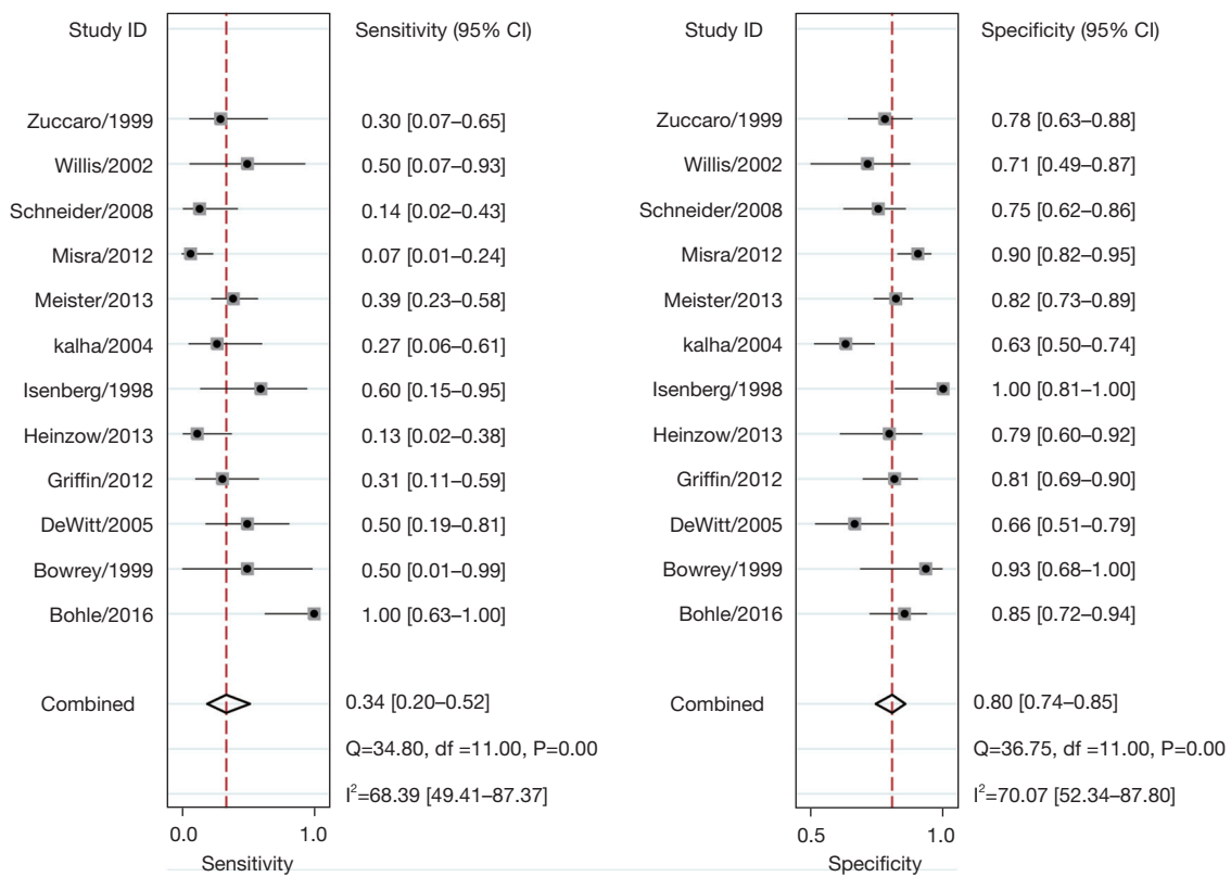
Figure 6 Forest plot of sensitivity and specificity of individual study and summary study on the diagnosis of T2 stage using EUS. CI, confidence interval; df, degree of freedom; EUS, endoscopic ultrasound.
