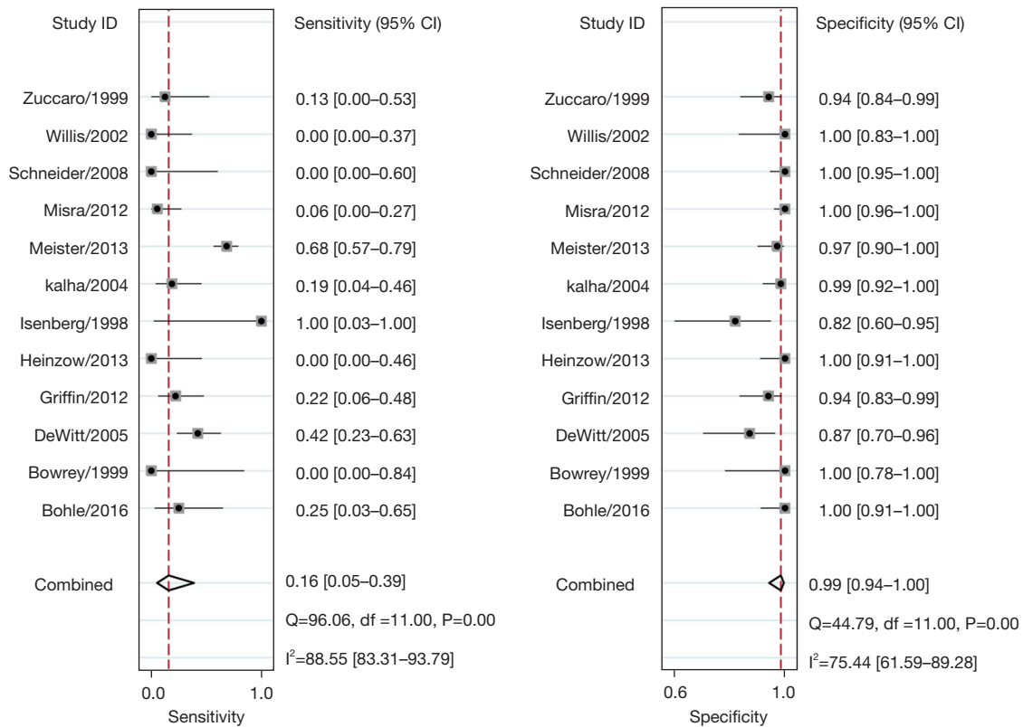
Figure 4 Forest plot of sensitivity and specificity of individual study and summary study on the diagnosis of T1 stage using EUS. CI, confidence interval; df, degree of freedom; EUS, endoscopic ultrasound.
