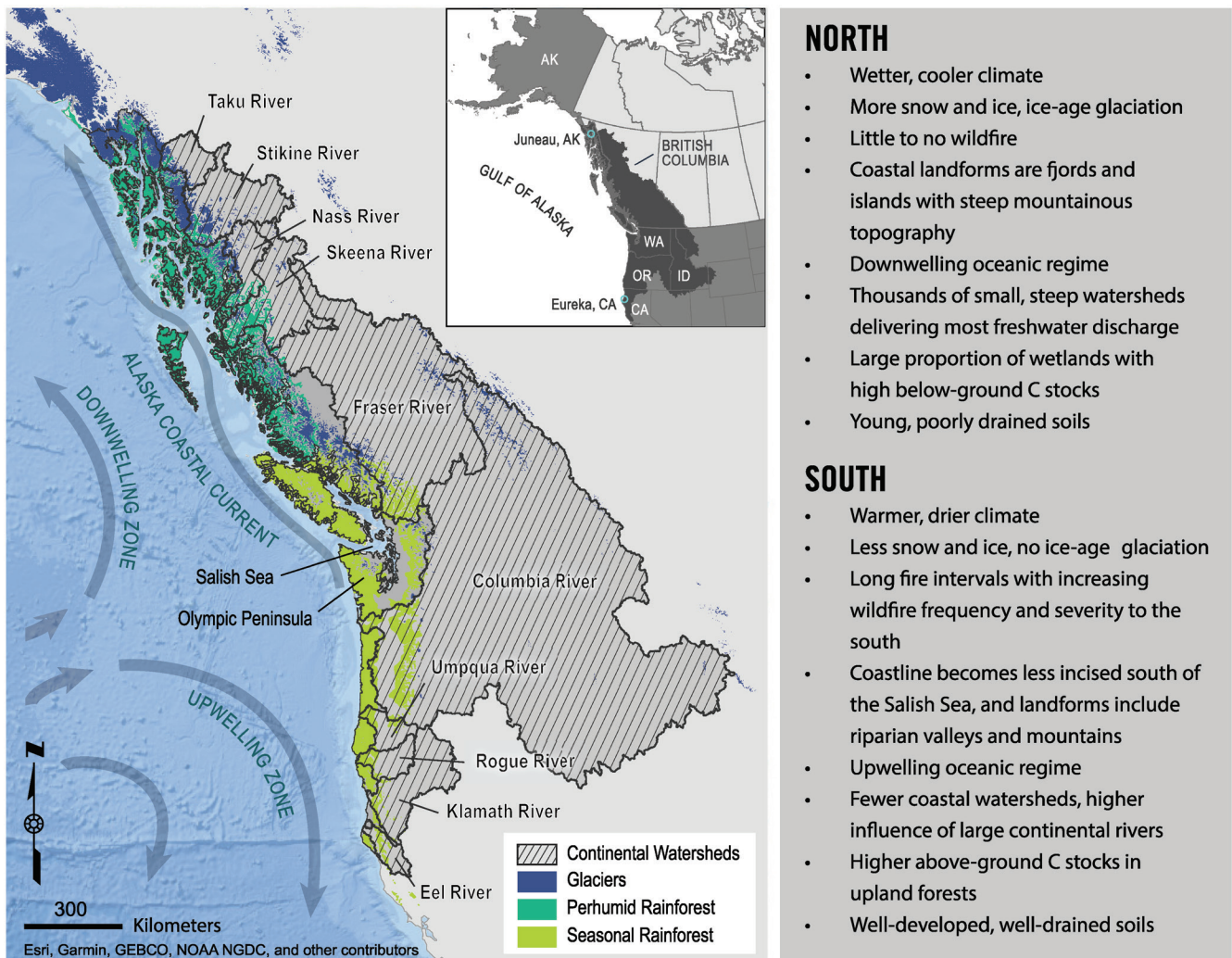
Figure 2. Map of the northeast Pacific coastal temperate rainforest (NPCTR) drainage basin (dark gray, inset) and perhumid and seasonal rainforest subregions. The ten largest watersheds are delineated with hash marks; these all have substantial portions of their basins outside of the NPCTR. The remainder of the drainage area is characterized by extensive rainforest cover and a large number of smaller watersheds (Gonzalez Arriola et al. 2018). Current ecosystem heterogeneity from north (perhumid rainforest) to south (seasonal rainforest) is described. Bathymetry is from Esri (2020). Source: Adapted from Kellogg (1995).
