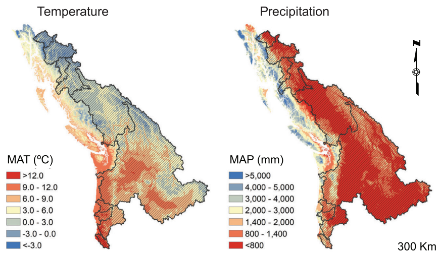
Figure 3. Regional climate normals (1981–2010) The outlines of the ten largest watersheds are shown with hash marks (Gonzalez Arriola et al. 2018). Source: The data are from Hamann et al. 2015, Wang et al. 2016). Abbreviations: MAP, mean annual precipitation; MAT, mean annual temperature.
