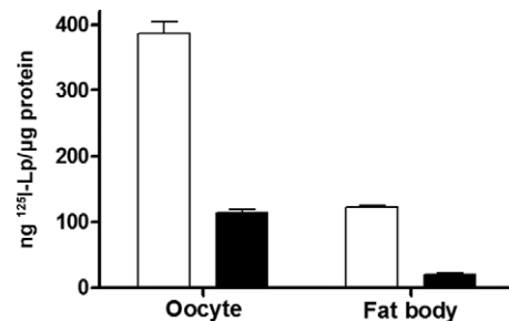
Fig. 1: comparative assay of lipophorin (Lp) binding to oocyte and fat body membranes. Specific binding of 125 I-Lp (40 \mu g/mL) to oocyte and fat body membrane preparations (40 \mu g protein/mL) was determined after 90 min of incubation in the presence of binding buffer (open bars). The non-specific binding (black bars) was determined in the presence of non-radioactive Lp (1.5 mg/mL). The results are expressed as ng bound 125 I-Lp/ \mu g of membrane protein and they are means and standard error of the means for four determinations. Other experimental conditions were as described in Materials and Methods.
