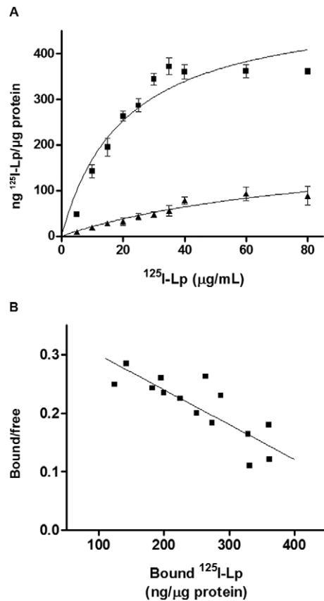
Fig. 4: determination of lipophorin (Lp) affinity for oocyte membranes. A: the oocyte membrane preparation (20 µg protein/mL) was incubated for 3 h with increasing concentrations of 125 I-Lp. The specific (■) and non-specific (▲) (in the presence of 1.5 mg/mL non-radioactive Lp) binding of 125 I-Lp to the membranes was determined. The results are expressed as ng bound 125 I-Lp/µg of membrane protein. The vertical bars represent the standard error of the means for four determinations and where they are not seen they are smaller than the symbols. Other experimental conditions were as described in Materials and Methods; B: Scatchard plot of the specific binding data from three different experiments. A K_d of 7.1 \pm 0.9 \times 10^{-8} M was calculated from three independent graphs.
