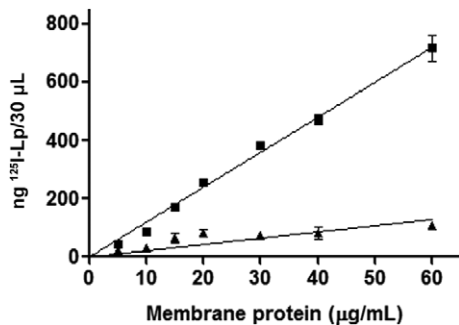
Fig. 3: effect of membrane protein concentration on the binding of lipophorin (Lp). 125 I-Lp (40 µg/mL) was incubated for 90 min with increasing concentrations of oocyte membrane protein and the specific (■) and non-specific (▲) (in the presence of 1.5 mg/mL non-radioactive Lp) binding of 125 I-Lp to the membranes was determined. The results are expressed as ng bound 125 I-Lp/30 µL of incubation medium. The vertical bars represent the standard error of the means for four determinations and where they are not seen they are smaller than the symbols. Other experimental conditions were as described in Materials and Methods.
