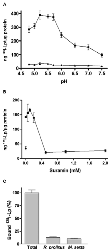
Fig. 5: effect of pH and suramin on lipophorin (Lp) binding to oocyte membranes and interaction specificity analysis. A: ^{125}\text{I} -Lp (40 \mu\text{g}/\text{mL} ) was incubated for 90 min with oocyte membrane preparation (20 \mu\text{g} protein/ \text{mL} ) at different pH values. The specific ( \blacksquare ) and non-specific ( \blacktriangle ) (in the presence of 1.5 \text{mg}/\text{mL} non-radioactive Lp) binding was determined; B: the total binding of ^{125}\text{I} -Lp (40 \mu\text{g}/\text{mL} ) to the oocyte membrane preparation (20 \mu\text{g} protein/ \text{mL} ) was determined in the presence of increasing concentrations of suramin ( \blacksquare ). The non-specific binding ( \blacktriangle ) was measured in the presence of non-radioactive Lp (1.5 \text{mg}/\text{mL} ) in the absence of suramin. In both graphics the results are expressed as ng bound ^{125}\text{I} -Lp/ \mu\text{g} of membrane protein. The vertical bars represent the standard error of the means for four determinations and where they are not seen they are smaller than the symbols; C: oocyte membrane preparation from Rhodnius prolixus was incubated with R. prolixus ^{125}\text{I} -Lp (40 \mu\text{g}/\text{mL} ) in the presence of an excess of non-radioactive Lp from R. prolixus or Manduca sexta (1.5 \text{mg}/\text{mL} ). Total binding of ^{125}\text{I} -Lp to the membranes was obtained in the absence of non-radioactive Lp. The results are expressed as percentages of total binding and they are means and standard error of the means for four determinations. Other conditions were as described in Materials and Methods.
