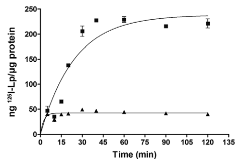
Fig. 2: time course of lipophorin (Lp) binding to oocyte membrane. 125 I-Lp (40 \mu g/mL) was incubated for different times with oocyte membrane preparation (20 \mu g protein/mL). The specific ( \blacksquare ) and non-specific ( \blacktriangle ) (in the presence of 1.5 mg/mL non-radioactive Lp) binding of 125 I-Lp to membranes was determined. The results are expressed as ng bound 125 I-Lp/ \mu g of membrane protein. The vertical bars represent the standard error of the means for four determinations and where they are not seen they are smaller than the symbols. Specific binding curve was built by a fitting of the data using one-phase exponential association equation with Prism 3.0 software. Other experimental conditions were as described in Materials and Methods.
