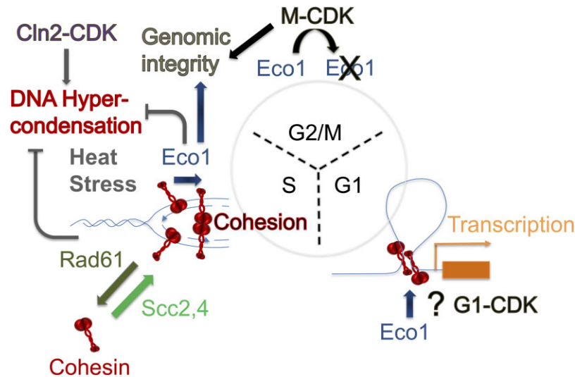
Fig. 7. Multifaceted and opposing roles for CDK regulation of Eco1 activity. In this current study, we provide evidence that Cln2-CDK regulates chromatin condensation reactions in combination with Eco1 and Rad61. Cln2-CDK promotes chromatin hypercondensation after START (possibly during S phase) and in response to thermic stress. Also during S phase, Eco1 establishes cohesion between cohesins newly deposited (via Scc2,4) onto nascent sister chromatids after passage of the DNA replication fork. Eco1 acetylation of cohesin (stabilizing cohesin dimers) blocks Rad61-dependent cohesin dissociation activities. After S phase, M-CDKs phosphorylate Eco1, resulting in Eco1 degradation through both G2 and M phases. In response to damage, however, Eco1 expression is significantly upregulated during G2/M to promote DNA damage-induced cohesion (not shown), even as Eco1 degradation continues. Intriguingly, eco1 is synthetically lethal in combination with either cdc28 (CDK) or cak (CDK activating kinase), revealing that Eco1 and M-CDK perform complementary roles to maintain genomic integrity (which are likely to include chromosome condensation, cohesion maintenance, and transcription regulation). During G1, Eco1 is critical for regulation gene transcription and genomic architecture within the nucleus. The role of G1-CDKs in this portion of the cell cycle remain largely unknown.
