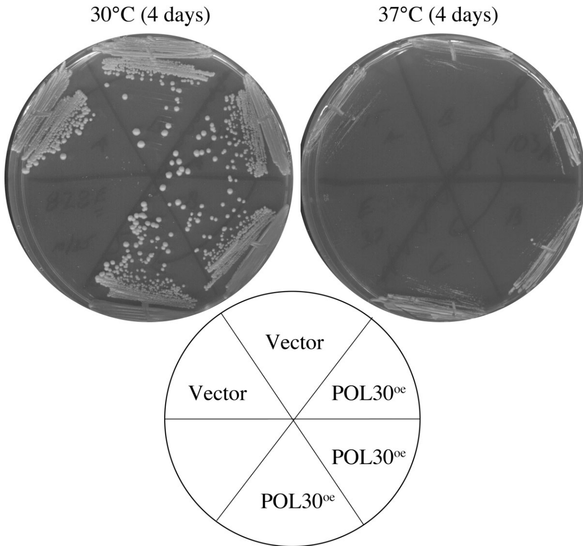
Fig. 4. Elevated expression of PCNA ( POL30 ) does not suppress eco1Δ rad61Δ mutant cell growth defects during thermic stress. The growth, 2 temperatures, of 2 independent isolates of eco1Δ rad61Δ double mutant cells transformed with vector alone compared to 3 independent isolates of eco1Δ rad61Δ double mutant cells transformed with vector that directs elevated POL30 expression.
