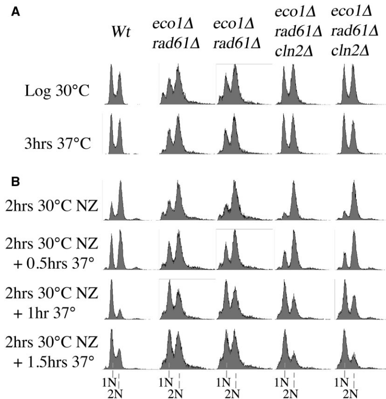
Fig. 5. Deletion of CLN2 does not delay, but instead promotes, cell cycle progression in eco1Δ rad61Δ mutant cells. a) DNA contents assessed using flow cytometry of log phase wildtype cells, 2 independent isolates of parental eco1Δ rad61Δ double mutant cells, and 2 independent isolates of eco1Δ rad61Δ cln2Δ triple mutant before and after growth at 37°C for 3 h. b) DNA contents of the cells, described in (a), released from a mitotic arrest (NZ, nocodazole) at the permissive temperature of 30°C then shifted to 37°C. Samples harvested every 30 min were analyzed for DNA content by flow cytometry.
