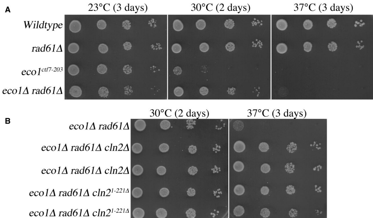
Fig. 1. Identification of the G1 cyclin, Cln2, as a regulator of Eco1-Rad61 pathways. a) eco1Δ rad61Δ double mutant cells are viable within a narrow temperature range. Ten-fold serial dilutions of wildtype, rad61Δ and eco1 ctf7-203 single mutant cells, and eco1Δ rad61Δ double mutant cells at the indicated temperatures. b) CLN2 deletion, and truncated Cln2 1-221 ( CLN2 1-221Δ ), both suppress eco1Δ rad61Δ double mutant cells growth defects. Ten-fold serial dilutions of wildtype cells, 2 independent isolates of eco1Δ rad61Δ cln2Δ triple mutant cells, and 2 independent isolates of eco1Δ rad61Δ cln2 1-221Δ cells grown at the indicated temperatures.
