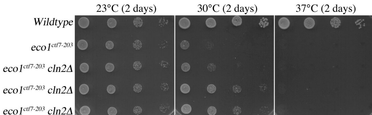
Fig. 3. Deletion of CLN2 suppresses eco1 mutant cell ts growth, similar to but distinct from deletion of RAD61 . Ten-fold serial dilutions of wildtype cells, eco1 ctf7-203 mutant cells, and 3 independent isolates of eco1 ctf7-203 cln2Δ double mutant cells grown at the indicated temperatures.
