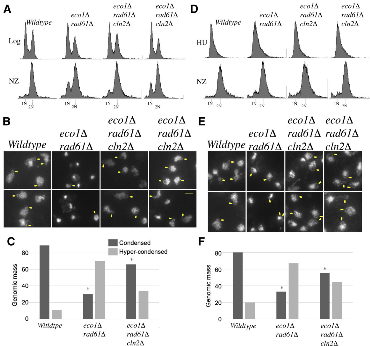
Fig. 6. Deletion of CLN2 rescues the chromatin hypercondensation defect otherwise present in eco1Δ rad61Δ cells under thermic stress. a) and d) DNA content of wildtype cells, parental eco1Δ rad61Δ double mutant cells, and 2 independent isolates of eco1Δ rad61Δ cln2Δ triple mutant at either log phase (a) or synchronized in S phase using HU (d), prior to growth for 3 h at 37°C in medium supplemented with nocodazole (NZ). b) and e) Micrographs of DNA masses and rDNA obtained from preanaphase cells as described in (a) and (d), respectively. Chromosomal masses and rDNA loop structures were detected using DAPI. White arrows indicate rDNA loops, which typically reside proximal to the genomic mass. c) and f) Quantification of genome mass areas, relative to template, for cells described in (a) and (d), respectively. For graph c: wildtype ( n = 38 ), eco1Δ rad61Δ ( n = 105 ), eco1Δ rad61Δ cln2Δ (2 replicates: n = 237 and n = 176 to produce an n_{\text{total}} = 413 ). For graph f: wildtype ( n = 117 ), eco1Δ rad61Δ ( n = 189 ), eco1Δ rad61Δ cln2Δ (2 replicates: n = 381 and n = 83 to produce an n_{\text{total}} = 464 ). Chi-squared tests were subsequently used to assess the dependence of gene mutations (* indicates P-value at or below 0.05) on chromatin condensation levels. For graph c: wildtype, P-value = 0.999; eco1Δ rad61Δ , P-value = 0.0000272; eco1Δ rad61Δ cln2Δ , P-value = 0.00104. For graph f: wildtype, P-value = 0.983; eco1Δ rad61Δ , P-value = 3.74 \times 10^{-14} ; eco1Δ rad61Δ cln2Δ , P-value = 4.45 \times 10^{-14} . Not shown: we also compared chromatin condensation effects across the 3 strains. The percentage of genomic masses, within a given field, that matched or exceeded the template was calculated and those values used to determine statistical significance: wildtype to eco1Δ rad61Δ , P = 0.00068; eco1Δ rad61Δ to eco1Δ rad61Δ cln2Δ (both replicates combined), P = 0.0066.
