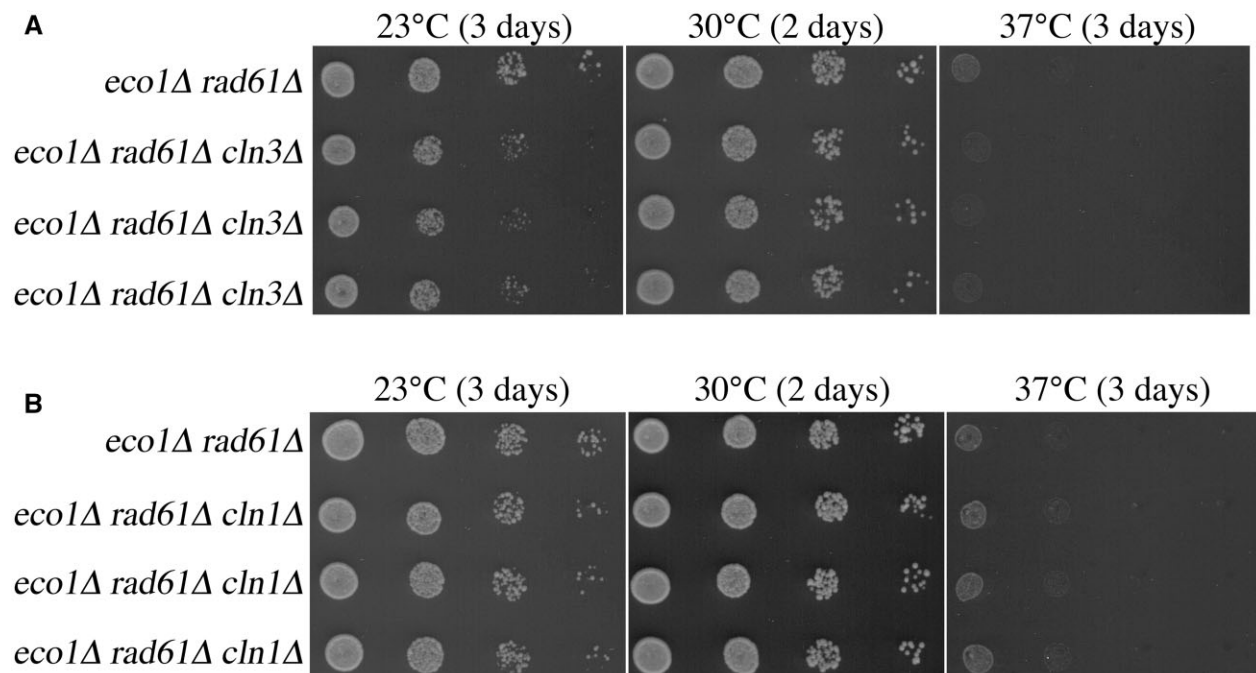
Fig. 2. The role of Cln2 in Eco1 - Rad61 functions is unique from Cln1 and Cln3 G1 cyclins. a) CLN3 deletion does not rescue eco1Δ rad61Δ cell growth defects under thermic stress. Ten-fold serial dilutions of parental eco1Δ rad61Δ double mutant cells and 3 independent isolates of eco1Δ rad61Δ cln3Δ triple mutant cells grown at the indicated temperatures. b) CLN1 deletion does not rescue eco1Δ rad61Δ cell growth defects under thermic stress. Ten-fold serial dilutions of parental eco1Δ rad61Δ double mutant cells and 3 independent isolates of eco1Δ rad61Δ cln1Δ triple mutant cells grown at the indicated temperatures.
