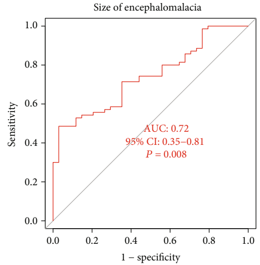
FIGURE 3: The predictive efficacy of encephalomalacia size on the prognosis of patients with refractory epilepsy secondary to encephalomalacia. AUC: area under the curve; CI: confidence interval.
