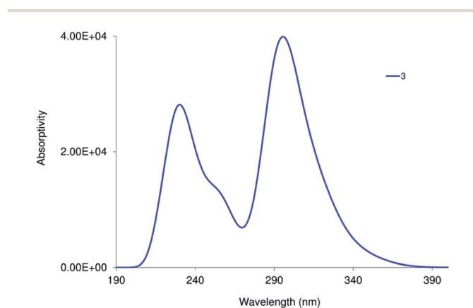
Fig. 4 Calculated electronic spectra of 3 at TD/PCM(DMSO)/CAM-B3LYP/LANL2DZ level of theory in the singlet state.
