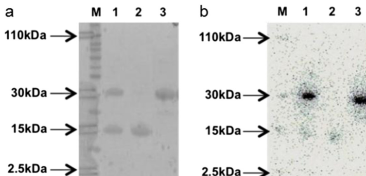
Figure 3 Specificity of [ 99m Tc(CO) 3 ] + to His-tagged protein was demonstrated via (a) SDS-PAGE followed by (b) phosphor imaging. Non-His-tagged protein (C2Ac, 15 kDa) was co-incubated with His-tagged protein (α-CD33 scFv, 29 kDa) and [ 99m Tc(CO) 3 ] + . The proteins were then separated using SDS-PAGE, and radiolabelling was visualised using phosphor imaging. Lanes M, molecular weight marker; lanes 1, C2Ac + α-CD33 scFv; lanes 2, C2Ac; lanes 3, α-CD33 scFv. Radioactive markers, indicated by black arrows, were placed at 2.5, 15, 30 and 110 kDa.
