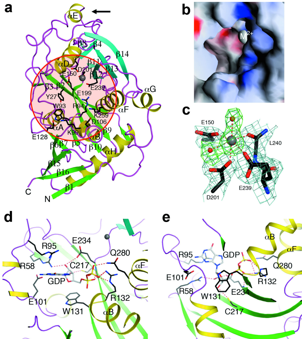
Figure 3. Structure of Rai1
