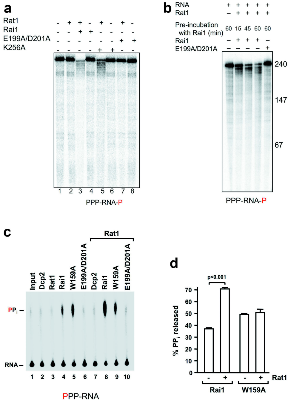
Figure 4. Biochemical evidence for pyrophosphohydrolase activity of Rai1
