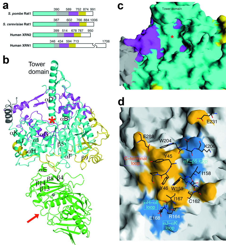
Figure 1. Structure of the Rat1-Rai1 complex
