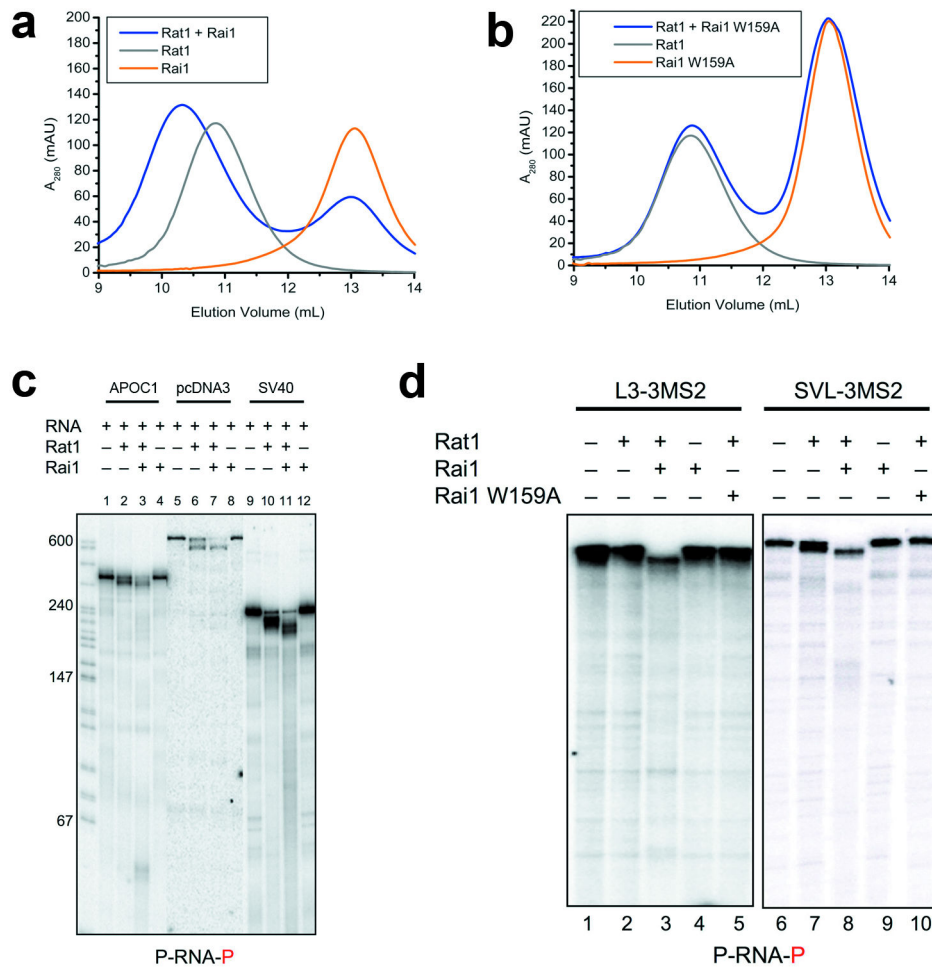
Figure 2. Biochemical and functional characterization of the Rat1-Rai1 interaction (a). Gel filtration profiles for wild-type Rat1 (full-length) alone, wild-type Rai1 (full-length) alone, and their mixture (with Rai1 present in roughly 2-fold molar excess). (b). Gel filtration profiles for wild-type Rat1 alone, W159A mutant of Rai1 alone, and their mixture. (c). Cleavage of three different 5' phosphorylated, 3' labeled RNA substrates by Rat1 and the Rat1-Rai1 complex. The RNA substrate is indicated at the bottom of the figure, with the radiolabeled phosphate group shown in red. (d). Cleavage of two other RNA substrates, each with three MS2 binding sites, by Rat1 and the Rat1-Rai1 complex.
