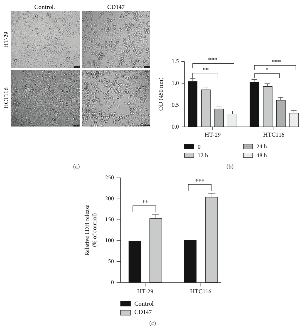
FIGURE 1: Effects of CD147 on pyroptosis. (a) Representative images of IECs ( \times 200 ) treated with CD147 (10 ng/mL) for 24 hours. Scale bar = 100 \mu\text{m} . (b) The CCK-8 assay was performed to detect cell viability in response to CD147 treatment for various time points. (c) The levels of LDH were measured by the LDH detection assay.
