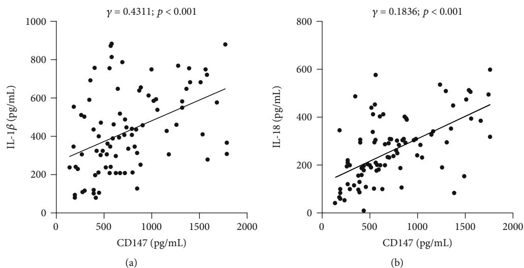
FIGURE 4: Clinical correlation between CD147 and IL-18 as well as IL-1 \beta . ELISA was used to examine the level of CD147, IL-18, and IL-1 \beta in serum from patients with inactive ( n = 19 ) or active ( n = 77 ) IBD. The clinical association was generated between CD147 and IL-1 \beta (a) and IL-18 (b).
