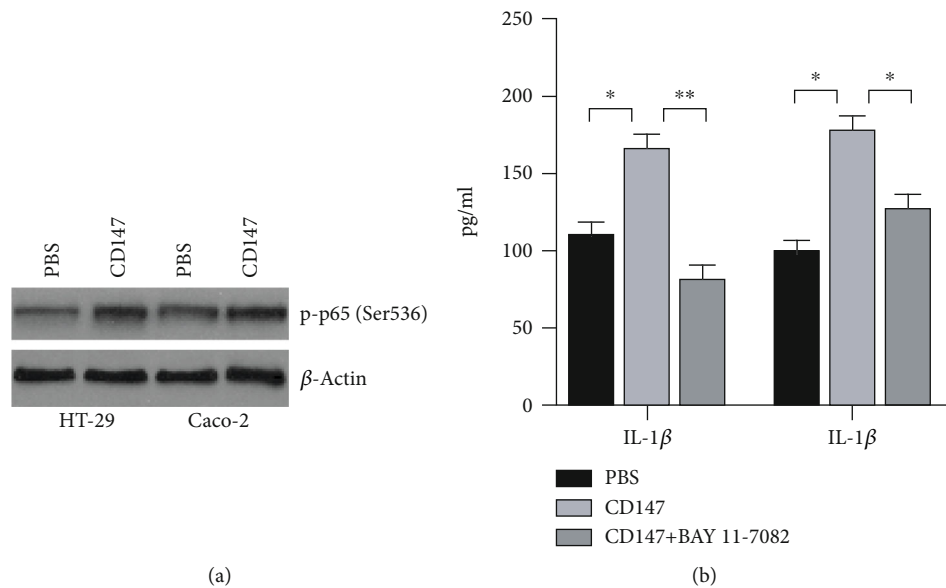
FIGURE 3: CD147 regulated IL-18 and IL-1 \beta expression in an NF- \kappa B-dependent manner. (a) Western blotting was performed to examine the phosphorylation of NF- \kappa B in HT-29 and Caco-2 cells. (b) ELISA was employed to examine IL-18 and IL-1 \beta secretion.
