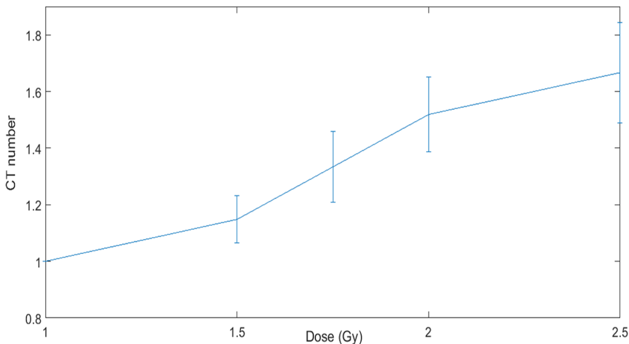
Figure 5: The computed tomography (CT) numbers with the dose for the NIPAM polymer gel dosimeter.
