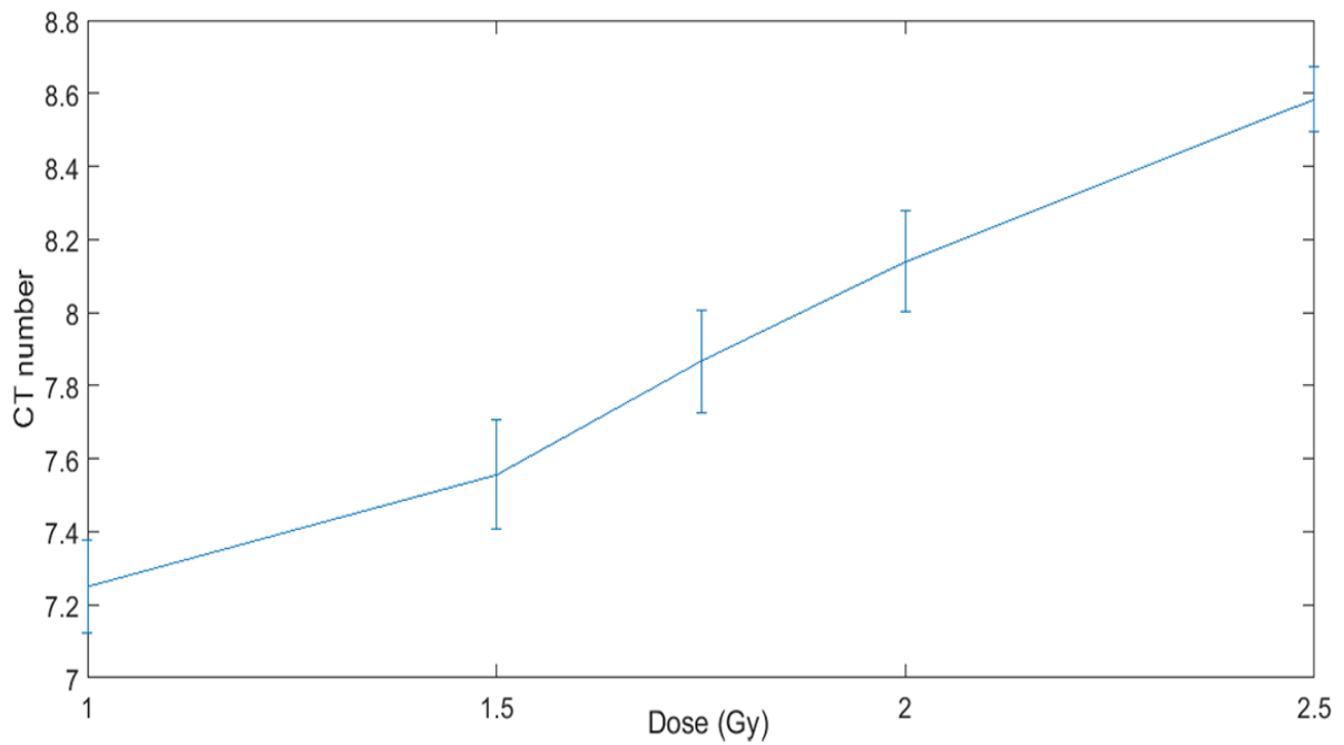
Figure 3: The computed tomography (CT) numbers with the dose for the new MAGAT polymer gel dosimeter.
