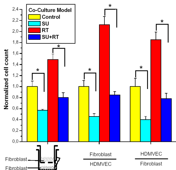
Figure 5 Co-culture experiments. Cells in lower compartments were selectively irradiated to induce paracrine proliferation of cells in upper compartments. Radiation (10Gy) of endothelial cells (HDMVECs) and fibroblast cells stimulated fibroblast proliferation (RT) in upper compartments. The administration of SU9518 significantly inhibited radiation-induced fibroblast proliferation. Likewise, irradiation of fibroblasts stimulated the proliferation of HDMVECs. The paracrine induction of endothelial cell proliferation was significantly inhibited by SU9518. The basal paracrine mitogenic stimulation of fibroblasts or endothelial cells in the upper compartment induced by co-culturing with non irradiated control cells in the lower compartment was also effectively inhibited by SU9518 (all SU9518 vs. control groups). Bars are mean \pm SD. In all figures asterisks indicate degree of statistical significance: *significant, P < 0.05 ; **highly significant P < 0.01 .
