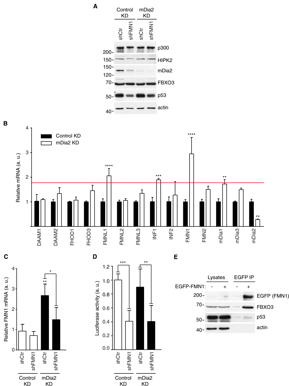
FIG. 5. mDia2 and FMN1 cooperate in the regulation of p53. A , Generation of control, mDia2, FMN1 and mDia2-FMN1 knockdown cells. 293T cells were infected with either control (Control KD ) or mDia2-targeting (mDia2 KD ) viruses. These cells were further infected with either control (shCtr) or FMN1-targeting (shFMN1) viruses. Total cell lysates were immunoblotted as indicated. One of two similar experiments is shown. B , Formin-expression landscape in control (Control KD ) and mDia2 knockdown (mDia2 KD ) cells. RT-qPCR analyses were performed using the indicated Formin-specific primers to determine relative expression levels (Relative mRNA, arbitrary units (a. u.)) ( n = 6 ; Two-way ANOVA). Cut-off red line is based on the fact that mDia1 silencing in mDia2 KD cells did not affect p53 activity (not shown). C , FMN1 silencing in mDia2 KD cells restores normal FMN1 expression. Cells were generated and total RNA obtained as in A and Fig. 4C, respectively. RT-qPCR shows the relative FMN1 levels (Relative FMN1 mRNA, arbitrary units (a. u.)) ( n = 6 ; One-way ANOVA). FMN1 down-regulation in the Control KD cells is not evident because of its very low basal expression. D , mDia2 and FMN1 cooperate in regulating p53 activity. Cells were plated, transfected and the luciferase activity measured and plotted as in B ( n = 6 ; One-way ANOVA). Similar results were obtained with a second FMN1-specific hairpin (not shown). E , Endogenous FBXO3 and p53 coprecipitate with EGFP-FMN1. 293T cells were transfected with either EGFP-tagged FMN1 (+) or the corresponding empty vector (-). Immunoprecipitation with GFP-trap beads was performed as described in the Experimental Procedures. Lysate (2%) and immunocomplexes (IP) were separated by SDS-PAGE and immunoblotted as indicated.
