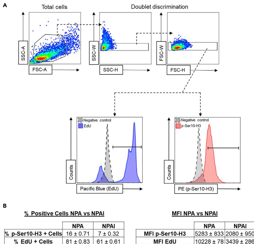
Figure 3. Flow Cytometry Gating Strategy Used to Identify EdU+ and p-Ser10-H3+ Glioma Cells
