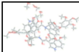
Fig. 1. The molecular structure of the main molecules, with atom labels and 50% probability displacement ellipsoids for non-H atoms. The crystal is a methanol solvate, with a 1:1 composition with respect to the main molecule. Solvent molecules were omitted.
