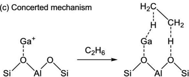
Scheme 2 Mechanism of ethane activation via (a) the alkyl mechanism, (b) the carbenium mechanism, and (c) the concerted mechanism. \text{Ga}^+ is a representative active site of \text{Ga/H-ZSM-5} .
