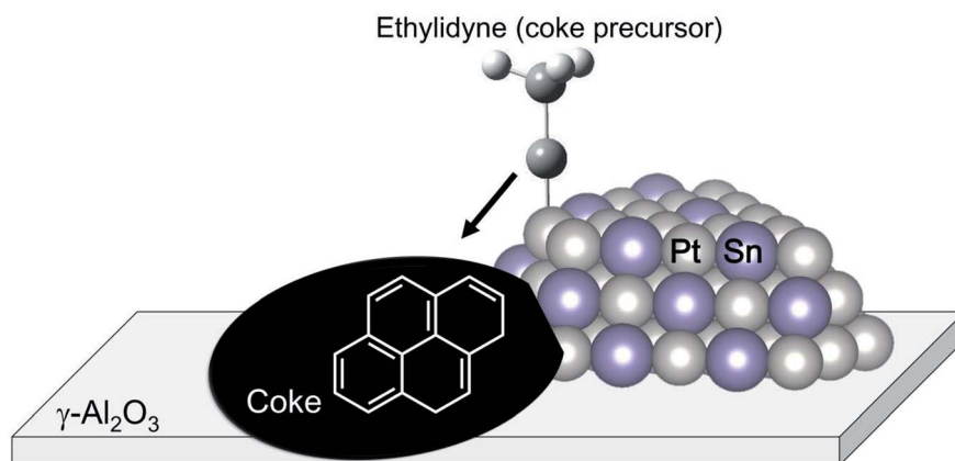
Fig. 7 Schematic image of the drain-off mechanism. Coke precursors such as ethylidyne move to the supports on which coke formation proceeds.
