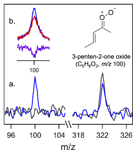
Fig. 1 (a) Mass spectra recorded with 118 nm photoionization of the (Z)-2,4-diiodo-pent-2-ene precursor (gray). Upon photolysis of the precursor at 248 nm in a 20% \text{O}_2/\text{Ar} carrier gas, the m/z 322 mass peak arising from the precursor ( \text{C}_5\text{H}_8\text{I}_2 ) is decreased and a new mass peak appears at m/z 100 with \text{C}_5\text{H}_8\text{O}_2 composition (blue), which is ascribed to the 3-penten-2-one oxide CI. (b) The m/z 100 photoionization signal (blue) decreases upon 410 nm ( ca. 4 mJ per pulse) excitation (red) with the difference trace (violet) illustrating the depletion signal. Also shown is the lowest energy tEE conformer of 3-penten-2-one oxide.
