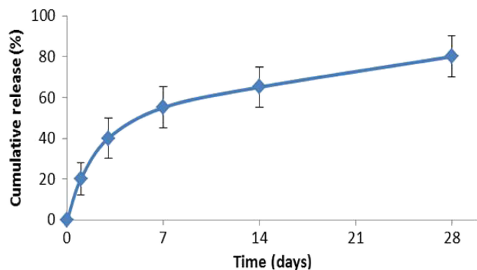
Figure 1. In-vitro drug release profile of Tetrilimus everolimus-eluting stent.
