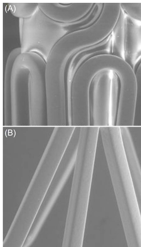
Figure 2. SEM images of (A) crimped and (B) expanded Tetrilimus stent.
