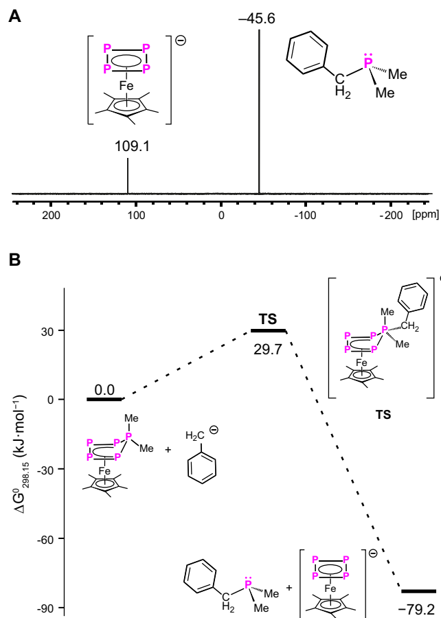
Fig. 5 Identification of the reaction pathway of phosphine abstraction. A Experimental 31 P{ 1 H} NMR (242.90 MHz, THF- d 8 ) spectrum of the crude reaction solution (low-temperature reaction) of 3c with KBnz at 180 K. B Gibbs free energy profile of the reaction of 3c with KBnz, calculated at the B3LYP-D3(BJ)/def2-TZVPP (PCM = THF) level of theory.
