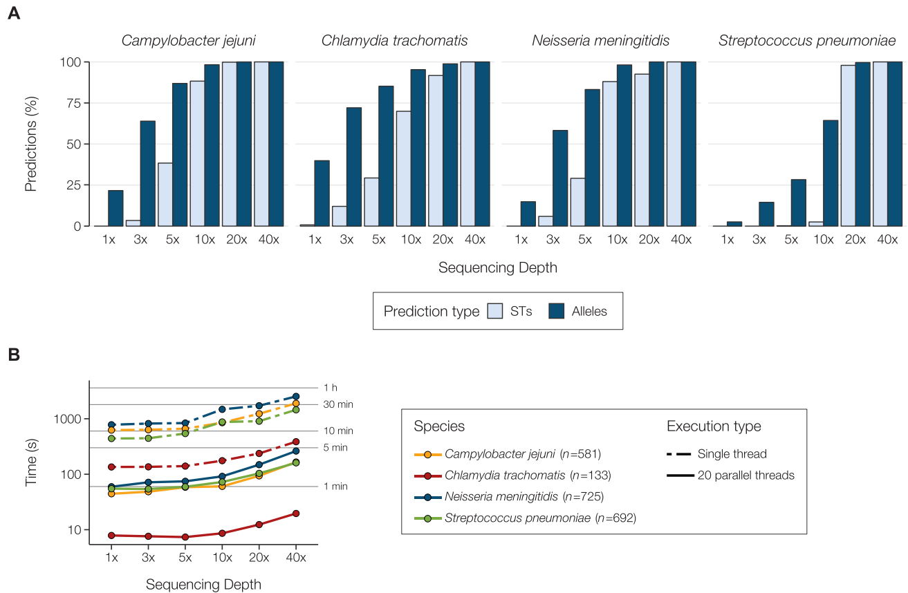
Figure 3. Results of the limit of detection test, and single- and multi-core performance test using MLST scheme. STing's sequence typing utility was run for MLST scheme in the fast mode over 1872 read samples simulated at 6 sequencing depths (1×, 3×, 5×, 10×, 20× and 40×) from assemblies of 4 species: Chlamydia trachomatis ( n = 133 ), Campylobacter jejuni ( n = 581 ), Neisseria meningitidis ( n = 725 ), and Streptococcus pneumoniae ( n = 433 ). (A) Percentage of correct predictions in terms of STs and alleles at different sequencing depths for the four datasets. (B) Total time in seconds (displayed in log-scale) required to process the complete dataset for each species at different sequencing depths using a single thread or instance (dashed lines) and 20 multiple threads (solid lines) of the sequence typing utility.
