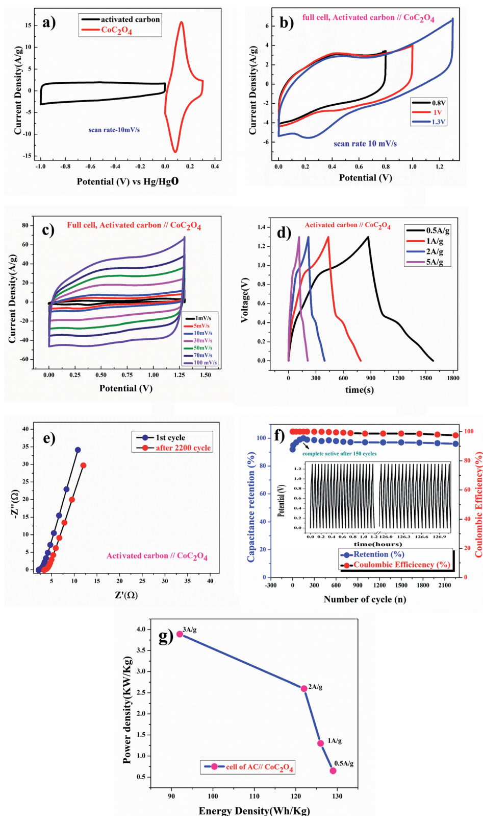
Fig. 8 Plot for activated carbon and porous anhydrous CoC 2 O 4 cell in ASC mode (a) CV at 10 mV s -1 , (b) full cell CV at 10 mV s -1 with different voltage window, (c) full cell CV at different scan rate, (d) charge–discharge, (e) EIS at 10 mV, (f) capacitance retention and coulombic efficiency and (g) power density and energy density.
