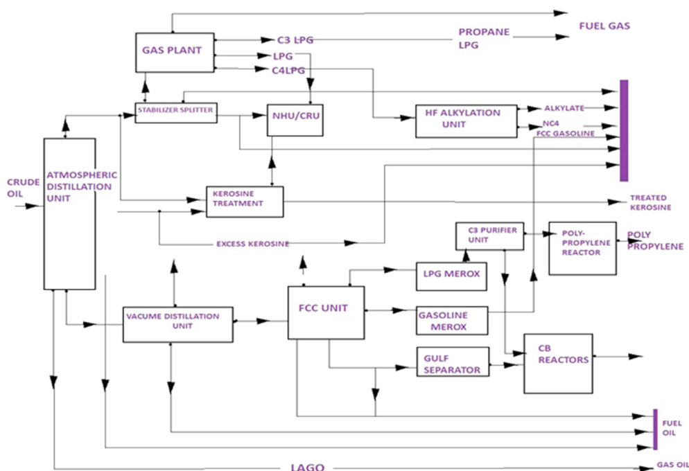
Figure 1. Block diagram of a typical petroleum refinery.
