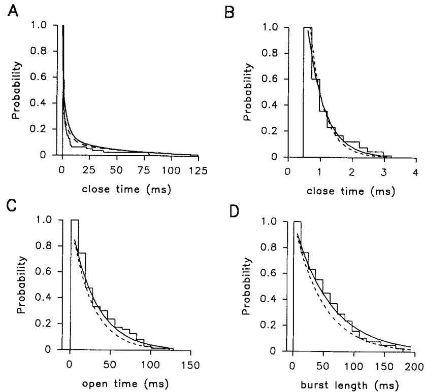
FIGURE 9. Closed-time, open-time, and burst length distributions at low PO_2 . (A) Cumulative histogram of closed-time intervals from records of the same experiment shown in Fig. 3 obtained while the patch was bathed in a hypoxic solution ( PO_2 \sim 5\text{--}10 mmHg). The continuous line is the distribution function fitted to the data ( \tau_1 = 0.44 ms, a_1 = 0.81 ; \tau_2 = 4.3 ms, a_2 = 0.14 ; \tau_3 = 46 ms, a_3 = 0.05 ; number of events = 81). The fitting obtained under normoxic conditions is also shown (dashed line) for comparison (see Fig. 3 B). These distributions were not statistically different (U test, \alpha > 0.05 ). (B) Cumulative histogram of closed events \leq 3 ms (see Fig. 3 C). The single exponential functions obtained in hypoxic (continuous line, \tau = 0.55 ms) and control (dashed line, \tau = 0.46 ms) conditions are superimposed on the histogram. Number of events = 66. Data were obtained from an inside-out patch with N = 1 K_{O_2} channel. Sampling interval = 250 \mu\text{s} ; imposed time resolution = 468 \mu\text{s} . Solutions: standard Na, TTX//130 K, 10 EGTA. (C and D) Open-time (C) and burst length (D) cumulative distributions in hypoxia during 400-ms pulses from -80 to +20 mV. Number of events = 61 and 38, respectively. The scaled single-exponential distribution functions are shown superimposed to the histograms. The fittings obtained under normoxic conditions (dashed lines) are also shown for comparison. Data were obtained from an inside-out patch with N = 1 K_{O_2} channel. Sampling interval = 250 \mu\text{s} ; imposed time resolution = 468 \mu\text{s} . Solutions: standard Na, TTX//130 K, 10 EGTA.
