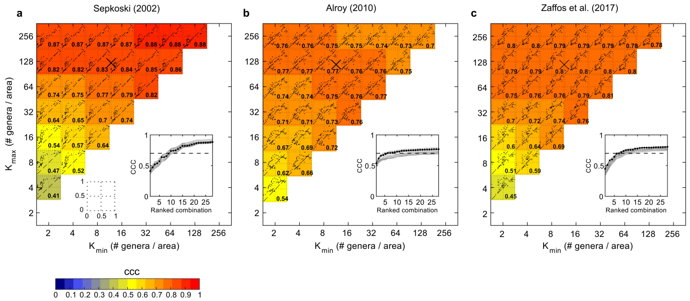
Extended Data Fig. 4 | Calibrating the logistic model's carrying capacities. a-c, Lin's concordance correlation coefficient (CCC) for the relationship between the global diversities resulting from the model and the fossil diversity estimates of Sepkoski 20 (n = 66 data points) (a), Alroy 21 (n = 60) (b), and Zaffos et al 22 (n = 69) (c) using different combinations of K_{\min} and K_{\max} in the model. Only the time series data between the end of one mass extinction and the beginning of the next were included in the analysis. Superimposed on each combination of K_{\min} and K_{\max} are the scatterplots of the normalized (0-1) diversity data (model vs fossil). The inset in each panel shows the CCCs in
