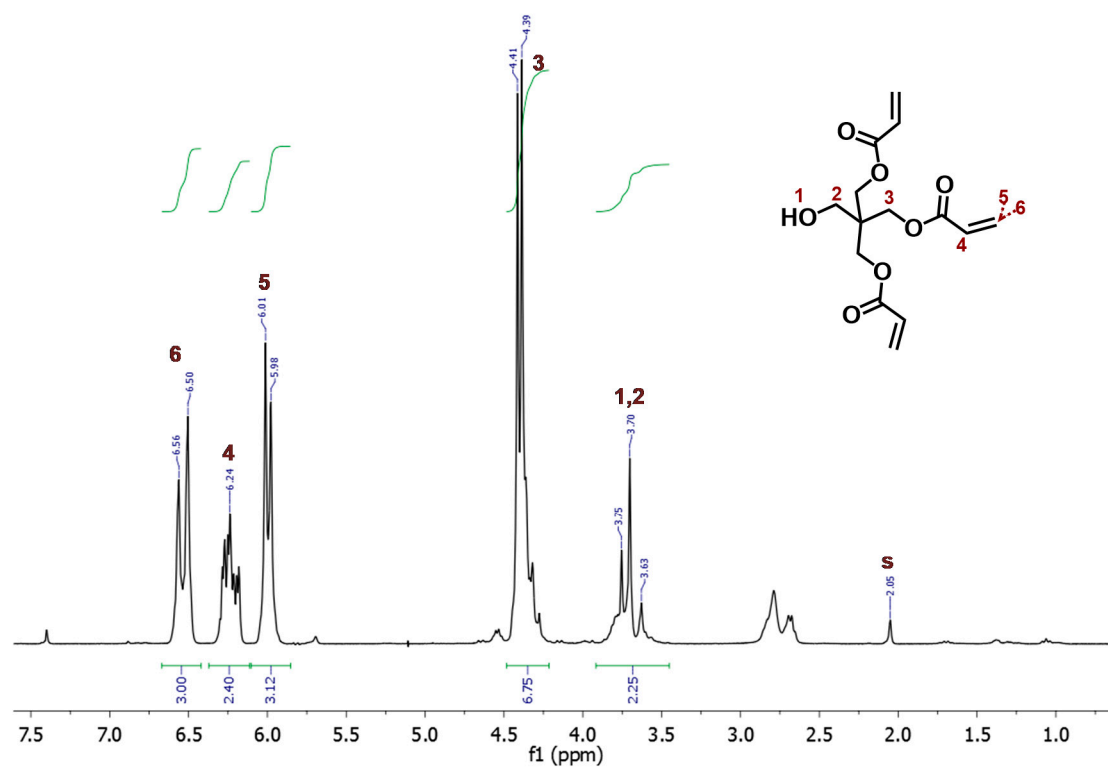
Figure 3. ^1\text{H-NMR} spectrum of SR444D in acetone- d_6 . The major component of this commercial product is pentaerythritol triacrylate (PETA), the peaks of which have been marked and integrated.
