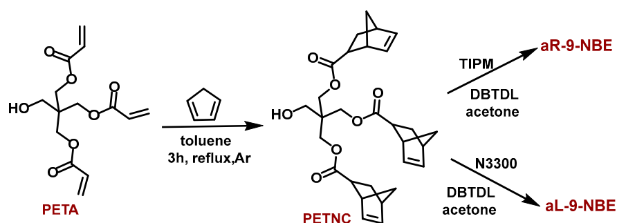
Scheme 2. Synthesis of dendritic monomers.
