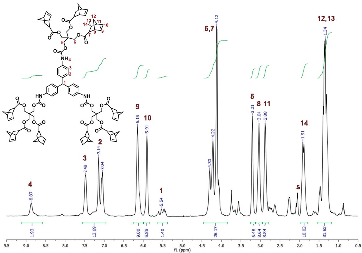
Figure 6. 1 H-NMR spectrum of aR-9-NBE in acetone-d 6 .
