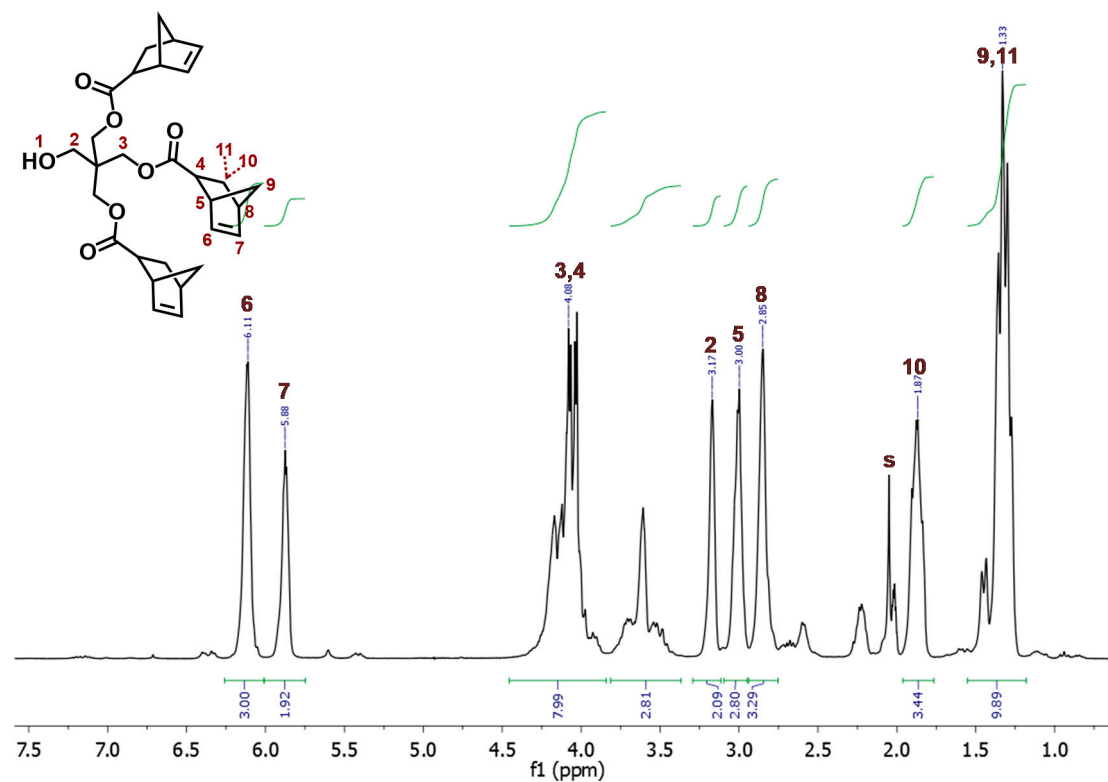
Figure 4. ^1\text{H-NMR} spectrum of pentaerythritol-norbornene-carboxylate (PETNC) in acetone- d_6 .
