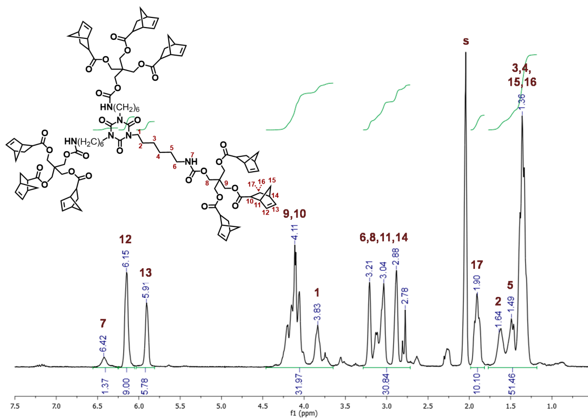
Figure 5. 1 H-NMR spectrum of aL-9-NBE in acetone-d 6 .
