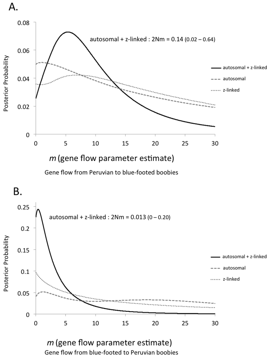
Figure 3. Posterior probability distributions from IMA [45] for gene flow between blue-footed and Peruvian boobies for the total, autosomal, and z-linked datasets. Gene flow parameters m_1 and m_2 scaled by the mutation rate. 2Nm = population migration rate per generation. A) Gene flow from Peruvian boobies to blue-footed boobies ( m_1 ). B) Gene flow from blue-footed boobies to Peruvian boobies ( m_2 ). doi:10.1371/journal.pone.0062256.g003
