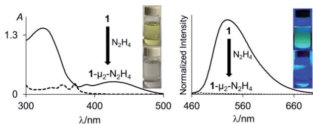
Fig. 3 UV-vis absorption (left) and emission (right) spectra of 1 (solid line) and 1-μ 2 -N 2 H 4 (dash line) ( 4.52 \times 10^{-5} M, \lambda_{\text{ex}} = 370 nm) in THF. The pictures of the solutions were taken at the same concentration. The images showing the fluorescence emission were illuminated with a hand-held UV lamp.
