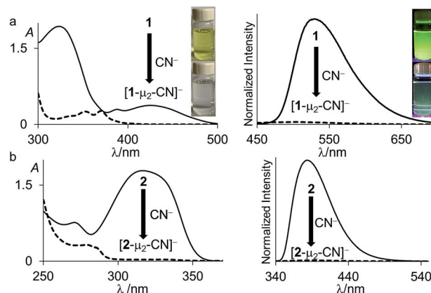
Fig. 4 UV-vis absorption (left) and emission (right) spectra of (a) 1 (solid line) and [1-μ 2 -CN] - (dash line) ( 6.91 \times 10^{-5} M, \lambda_{\text{ex}} = 370 nm) and (b) 2 (solid line) and [2-μ 2 -CN] - (dash line) ( 6.22 \times 10^{-5} M, \lambda_{\text{ex}} = 280 nm) in CHCl 3 /MeOH (1/1 vol). The pictures of the solutions were taken at the same concentration. The images showing the fluorescence emission were illuminated with a hand-held UV lamp.
