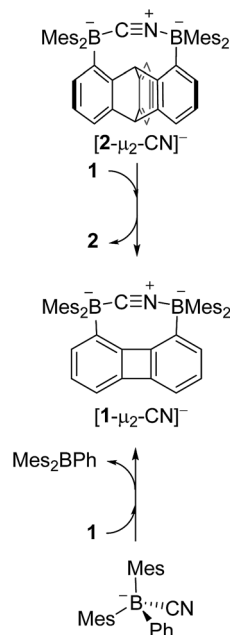
Scheme 6 Competition reactions of [\text{tBu}_4\text{N}][2-\mu_2\text{-CN}] and 1 (top) and [\text{tBu}_4\text{N}][3-\text{CN}] and 1 (bottom). The [\text{tBu}_4\text{N}]^+ cations are not shown for clarity.
