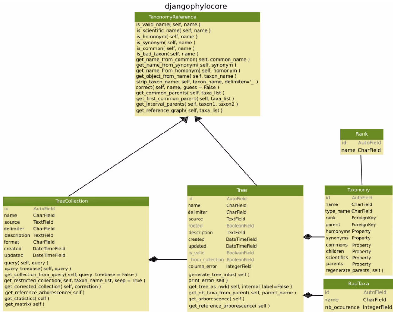
Figure 1 UML diagram of the PhyloCore library structure of PhyloExplorer.
