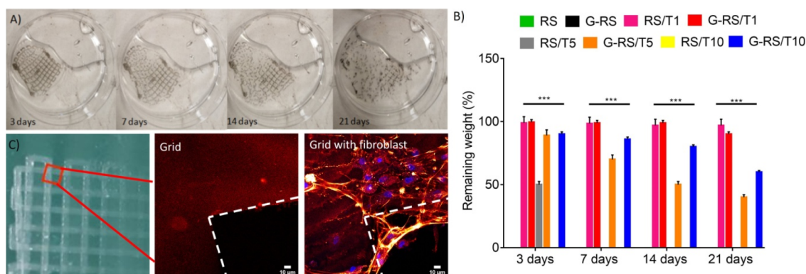
Figure 10. (A) Photographs of the bioresorbable 3D printed grid ( i.e. , G-RS/T10) in PBS solution ( i.e. , 37 ^\circ\text{C} , pH 7.4) and (B) measurements of the rates of dissolution obtained on films. (C) Confocal microscopy images of human fibroblasts seeded on the RS grid. Images were taken at grid intersections. The scale bar indicates 10 \mu\text{m} . The autofluorescence of the grid allows us to highlight the growth of fibroblasts, in which the nuclei (blue) and the plasma membrane (red) are labeled.
