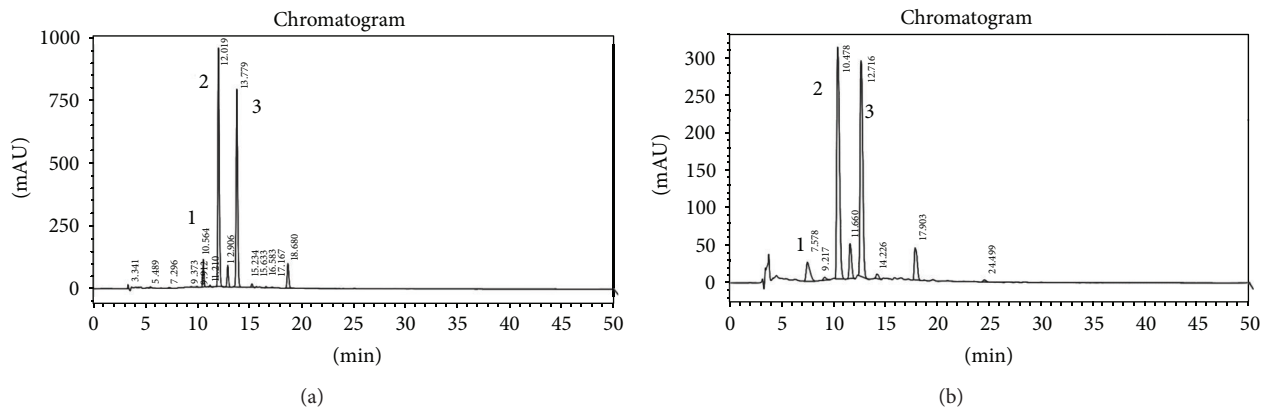
FIGURE 1: Anthocyanins profile. HPLC-UV chromatograms of fermented blueberry, (a) corresponds to the anthocyanins profile at the beginning of the fermentation process and (b) corresponds to the anthocyanins profile at the end of the fermentation process. Peak identification: 1, Delphinidin 3-glucoside; 2, cyanidin-3-glucoside; 3, petunidin-3-glucoside. Chromatographic analysis was carried out using a column Zorbax C18 and mixtures of acetonitrile/formic acid/water as mobile phase. The flow rate was 0.8 mL/min and detection was measured at 525 nm.
