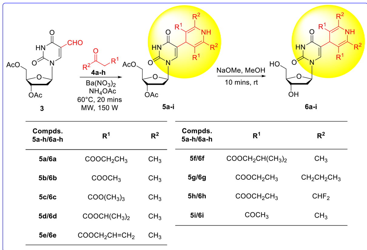
Scheme 2 Synthesis of fluorescent 1,4-dihydropyridine nucleoside analogues.
