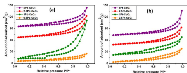
Fig. 3 The \text{N}_2 sorption isotherms of the prepared (a) Pd– \text{CeO}_2 and (b) Pt– \text{CeO}_2 .
