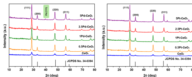
Fig. 2 XRD patterns of the prepared (a) Pd– \text{CeO}_2 , and (b) Pt– \text{CeO}_2 samples.
