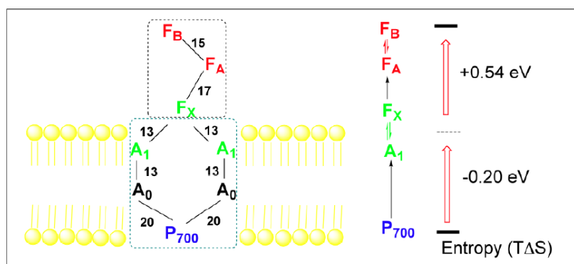
Figure 6. Thermodynamic and kinetic assignments of photoacoustic measurements in PS I of Synechocystis sp. PCC 6803 (reproduced with permission from the American Chemical Society [40]).
