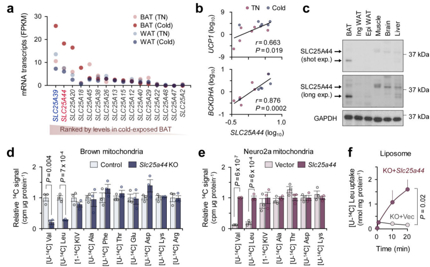
Figure 3. Identification of SLC25A44 as a mitochondrial BCAA transporter. a. Expression profile of SLC25A family members in human supraclavicular BAT and abdominal subcutaneous WAT from the same individual at 27°C and 19°C 5 . b. Correlation of SLC25A44 mRNA expression with UCP1 or BCKDHA in human BAT. Expressions at TN (red) and cold (blue) from 6 biological independent subjects. Pearson’s correlation coefficient was calculated. c. Protein expression of SLC25A44 in indicated tissues of mice. GAPDH as a loading control. Representative result from two independent experiments. Gel source data are in Supplementary Figure 1. d-e. Mitochondrial uptakes of indicated molecules in control and Slc25a44 KO brown adipocytes ( d ) or in Neuro2a cells expressing Slc25a44 or an empty vector ( e ). n = 3 /group, biologically independent samples. f. [ U-^{14}C_6 ] Leu transport into mitochondrial-liposomes from Slc25a44 KO brown adipocytes expressing an empty vector (KO+vector) or Slc25a44 (KO+ Slc25a44 ). n = 3 /group, technically independent samples. Representative result from two independent experiments. Mean \pm s.e.m.; two-sided P -values by unpaired Student’s t -test ( d , e ) or two-way ANOVA ( f ).
