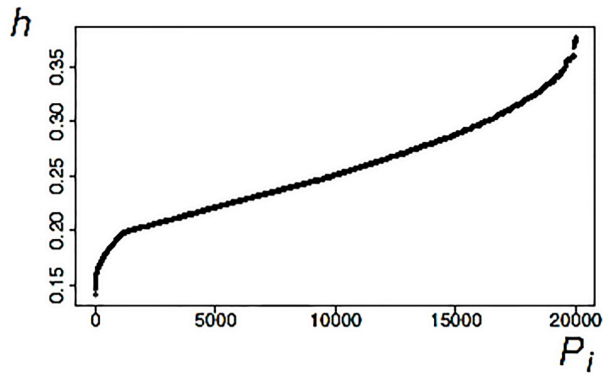
(a) Ranked h distribution versus P_i^{\text{out}} for \mathcal{G}_1 .
