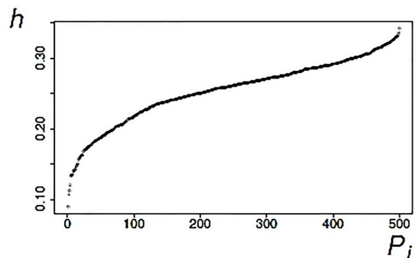
(f) Ranked h distribution versus P_i^{\text{in}} for \mathcal{G}_2^2 .
