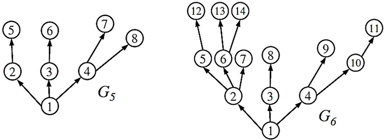
(a) G_5 with |V| = 8, |E| = 7 .
