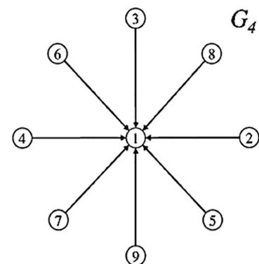
(b) G_4 with \min(I_1) where \max(I_2), G = (V, E), |V| = 9, |E| = 8 .
