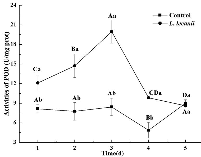
Figure 5 Effects of POD activities of the 3rd-instar B. tabaci nymphs infested with L. lecanii JMC-01. Times marked with different uppercase letters on the same line are significantly different ( P < 0.05 ). The different lowercase letters indicate significant differences between the treatment and control groups ( P < 0.05 ) at the same time point. Full-size DOI: 10.7717/peerj.7690/fig-5
