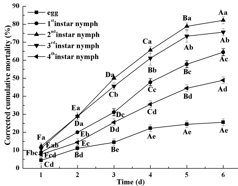
Figure 2 Cumulative corrected mortality of L. lecanii JMC-01 infestation on B. tabaci nymphs. Times marked with different uppercase letters on the same line are significantly different ( P < 0.05 ). The different lowercase letters indicate significant differences between the treatment and control groups ( P < 0.05 ) at the same time point.
