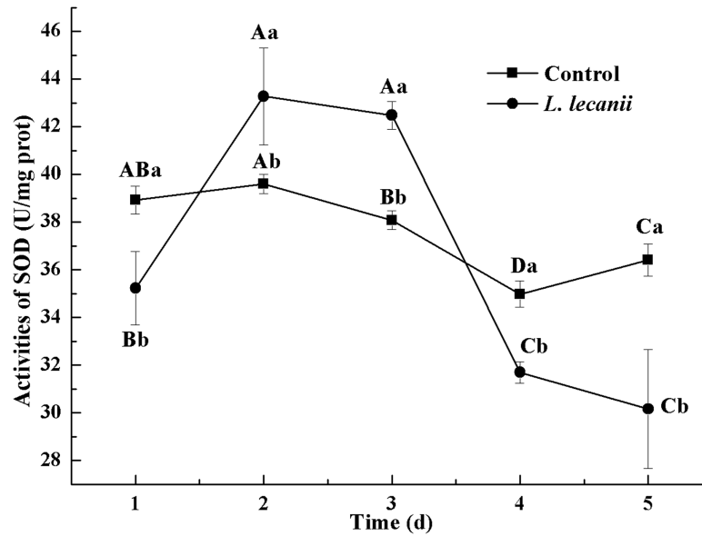
Figure 4 Effects of SOD activities of the 3rd-instar B. tabaci nymphs infested with L. lecanii JMC-01. Times marked with different uppercase letters on the same line are significantly different ( P < 0.05 ). The different lowercase letters indicate significant differences between the treatment and control groups ( P < 0.05 ) at the same time point. Full-size DOI: 10.7717/peerj.7690/fig-4
