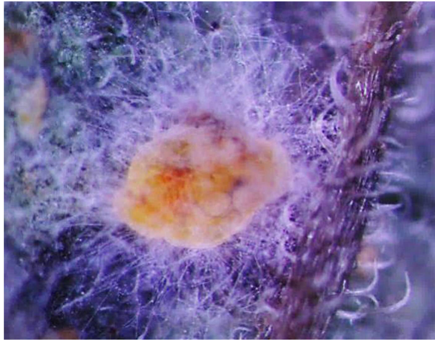
Figure 1 Morphological characteristics of the B. tabaci nymph induced by L. lecanii JMC-01.
